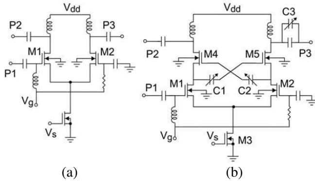
Figure 1. Schematics of (a) a conventional active balun; (b) the proposed active balun.
