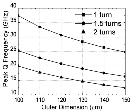
Figure 4. Inductor peak Q frequency versus the outer dimension and number of turns.
