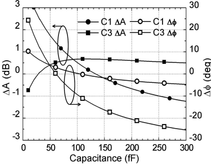
Figure 2. Amplitude and phase imbalance versus C1 and C3 capacitance.
