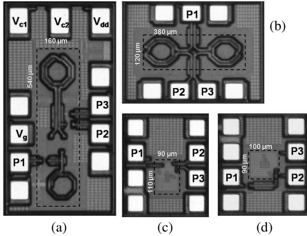
Figure 8. Chip micrograph of (a) active balun; (b) lumped-element balun; (c) transformer balun T1; (d) transformer balun T2.
