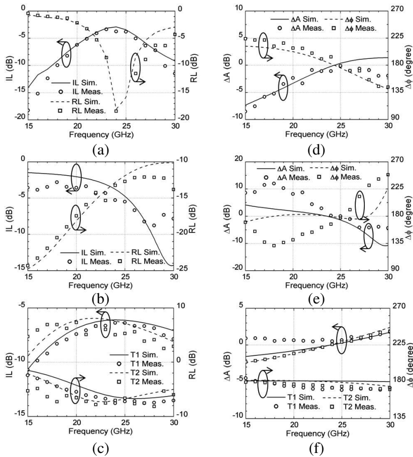
Figure 9. IL and RL of (a) the active balun; (b) the L-C balun; (c) the transformer baluns. \Delta A and \Delta\phi of the (d) the active balun; (e) the L-C balun; (f) the transformer baluns.
