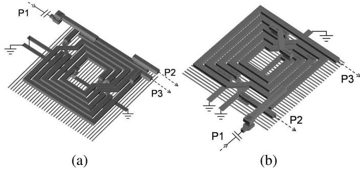
Figure 5. Layout of the transformer baluns.
