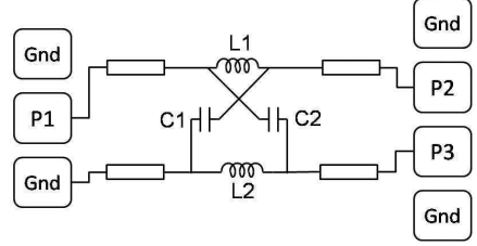
Figure 3. Layout of the transformer baluns.
