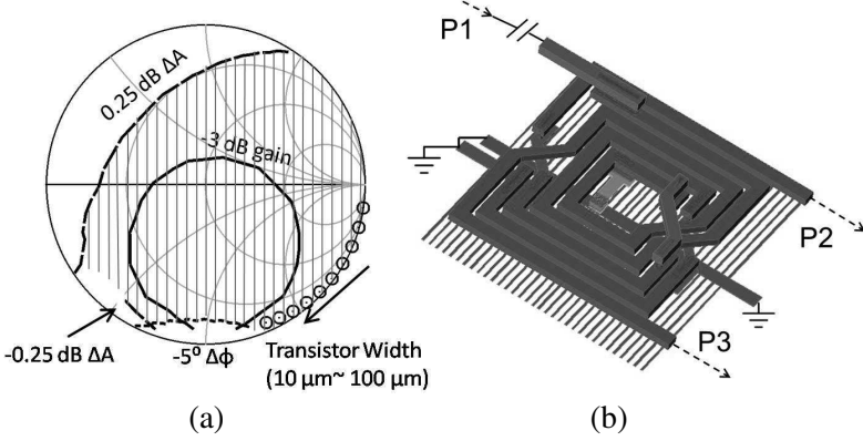
Figure 7. (a) Load impedance tuning for the modified transformer balun; and (b) layout of the modified balun.
