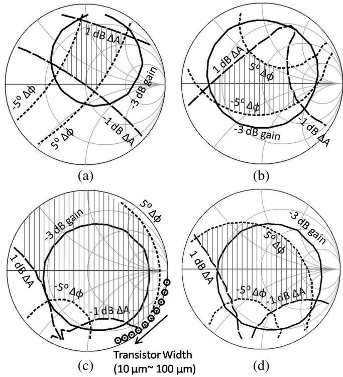
Figure 6. Load impedance tuning for (a) active balun; (b) L-C balun; (c) transformer balun T1; (d) transformer balun T2.
