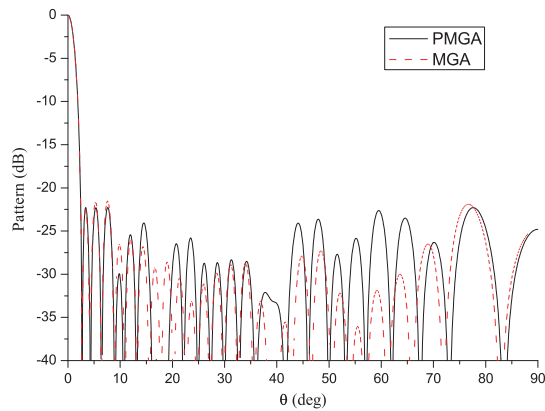
Figure 5. Best radiation patterns obtained by PMGA and MGA.
