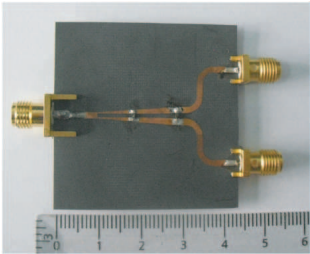
Figure 7. Photograph of the proposed power divider.
