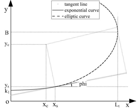
Figure 2. The structure geometry for the tapered line.
