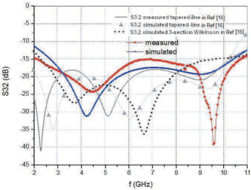
Figure 8. Comparisons of the isolation performance.
