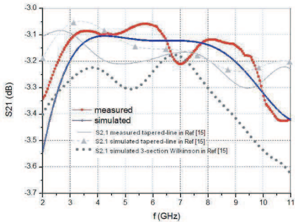
Figure 11. Comparisons of the transmission coefficient.
