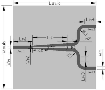
Figure 1. Geometry of the proposed power divider.
