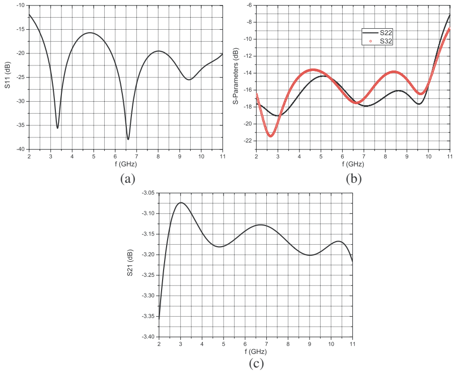
Figure 6. S -parameters of the power divider.
