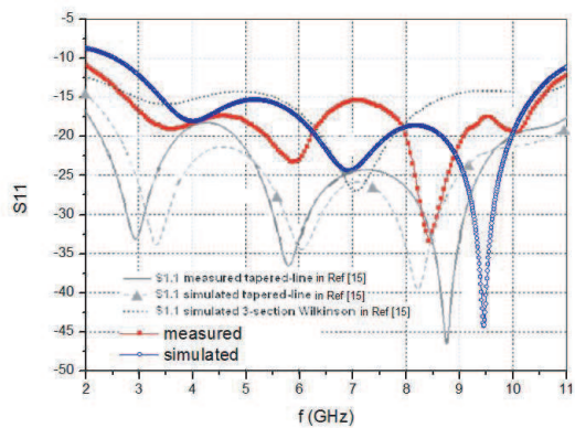
Figure 9. Comparisons of the return loss for port 1.
