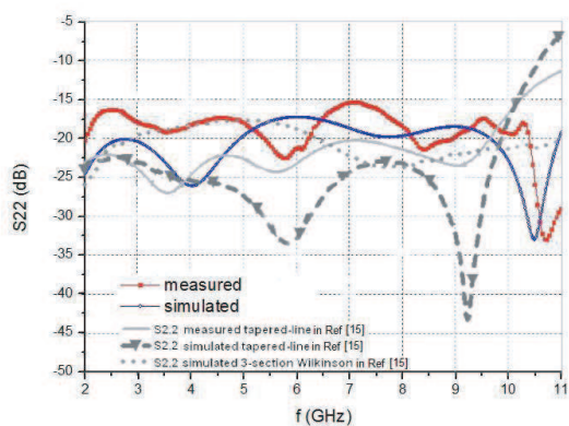
Figure 10. Comparisons of the return loss for port 2.
