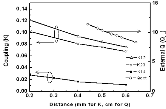
Figure 5. Values of k for different separation distances ( d ) and external coupling values ( Q_{ext} ) for different values of D .
