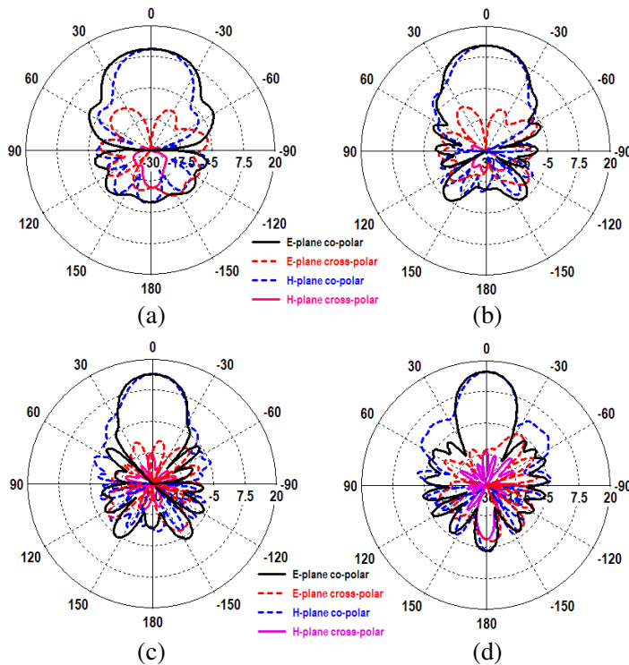
Figure 13. Simulated far field radiation patterns of the proposed AVA with NIM (multiple layers) at: (a) 9.5 GHz, (b) 12 GHz, (c) 16 GHz, and (d) 19.5 GHz.
