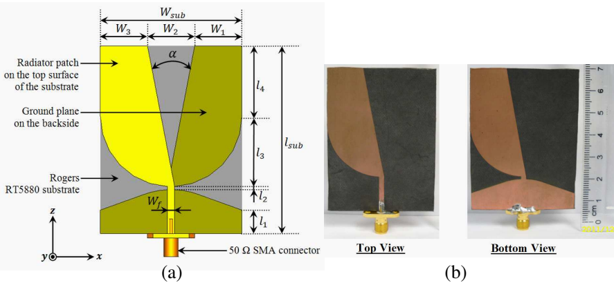
Figure 1. (a) Antenna geometry and (b) photograph.
