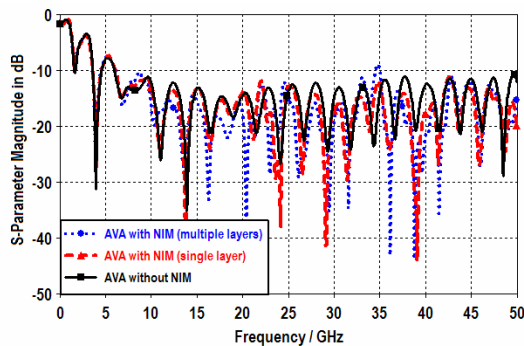
Figure 8. Simulated return loss of the AVA with and without NIM.
