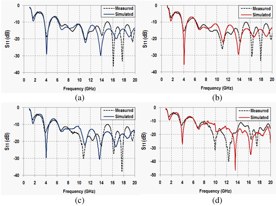
Figure 9. Measured and simulated return loss of the modified AVA: (a) without slit and NIM, (b) with slit, (c) with NIM (single layer), and (d) with NIM (multiple layers).
