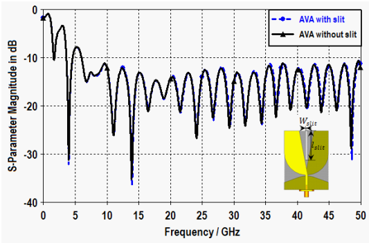
Figure 6. Simulated return loss of the modified AVA with and without slit.
