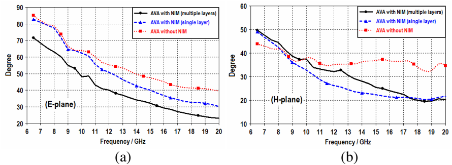
Figure 11. Simulated (a) angular width ( E -plane), and (b) angular width ( H -plane).
