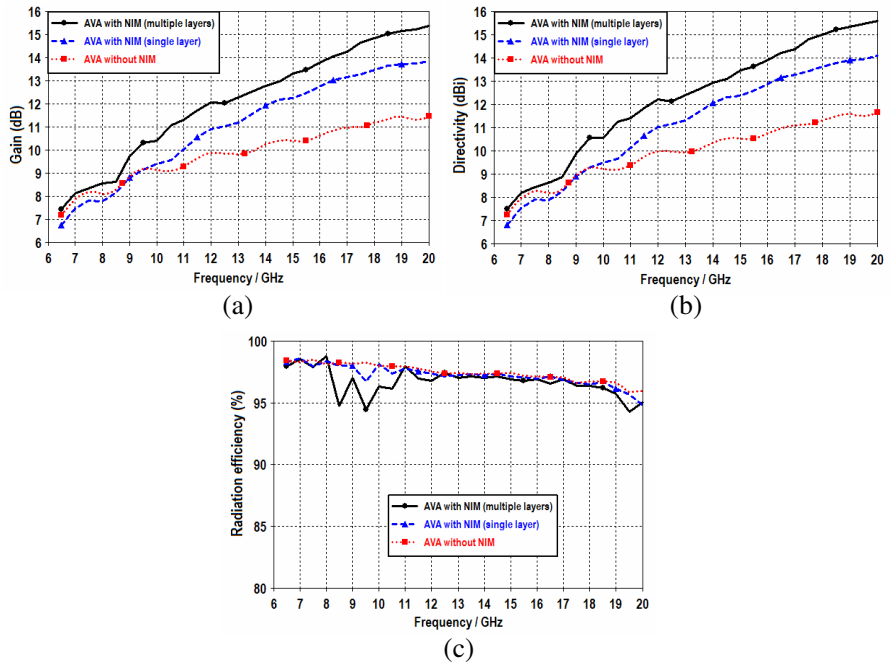
Figure 10. Simulated (a) gain, (b) directivity, and (c) radiation efficiency.
