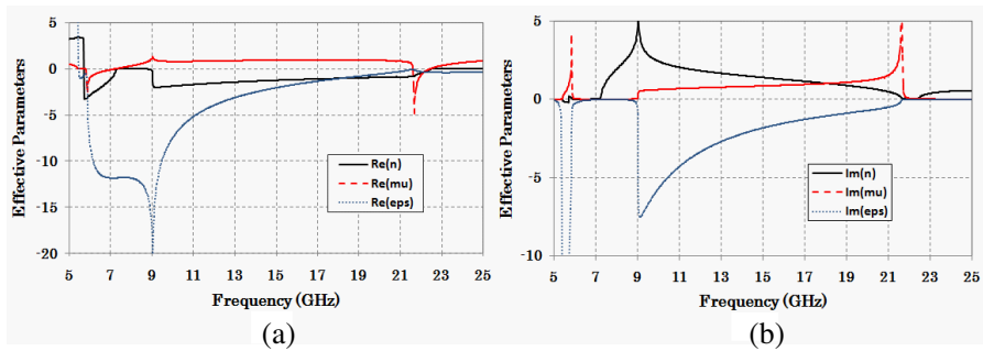
Figure 5. Retrieved effective parameters, (a) real parts and (b) imaginary parts.
