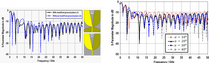
Figure 2. Return loss result of the proposed antenna with and without modified ground plane. Figure 3. Simulated return loss of the proposed AVA for different values of \alpha .
