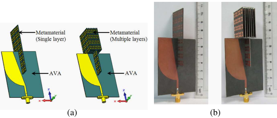
Figure 7. (a) The proposed AVA incorporated with NIM and (b) photograph.
