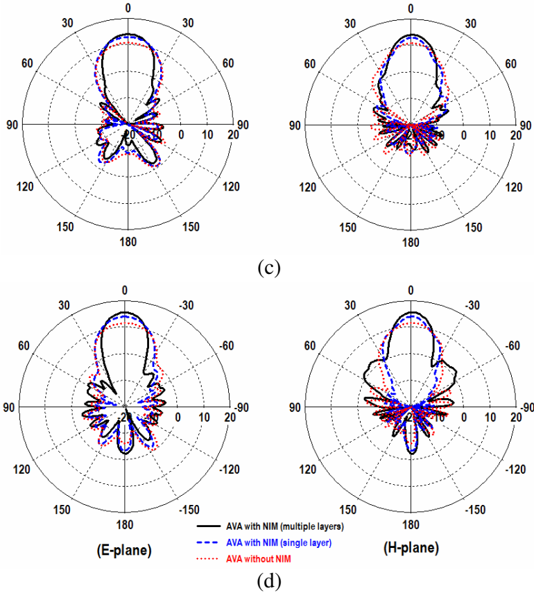
Figure 12. Comparison for simulated E -plane ( x - z ) and H -plane ( y - z ) radiation patterns of the antennas at: (a) 9.5 GHz, (b) 12 GHz, (c) 16 GHz, and (d) 19.5 GHz.
