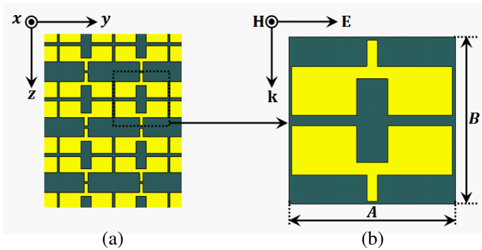
Figure 4. (a) NIM configuration and (b) its unit cell [14].
