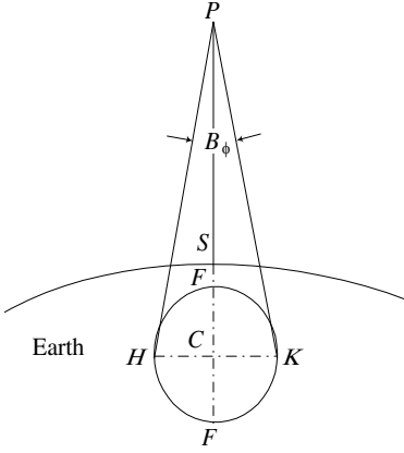
Figure 1. SP cell footprint.
