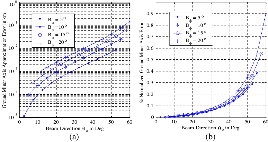
Figure 7. (a) Absolute error variation with beam direction at different beamwidths. (b) Relative error variation with beam direction at different beamwidths.
