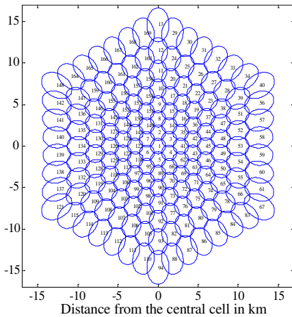
Figure 12. SP cellular layout constructed by 169 cell using 20 \times 20 antenna array.
