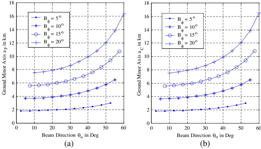
Figure 6. (a) a_F variation with beam direction at different beamwidths. (b) a_C variation with beam direction at different beamwidths.
