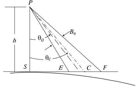
Figure 2. Flat ground approximation geometry.
