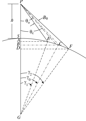
Figure 3. Curved earth coverage geometry.
