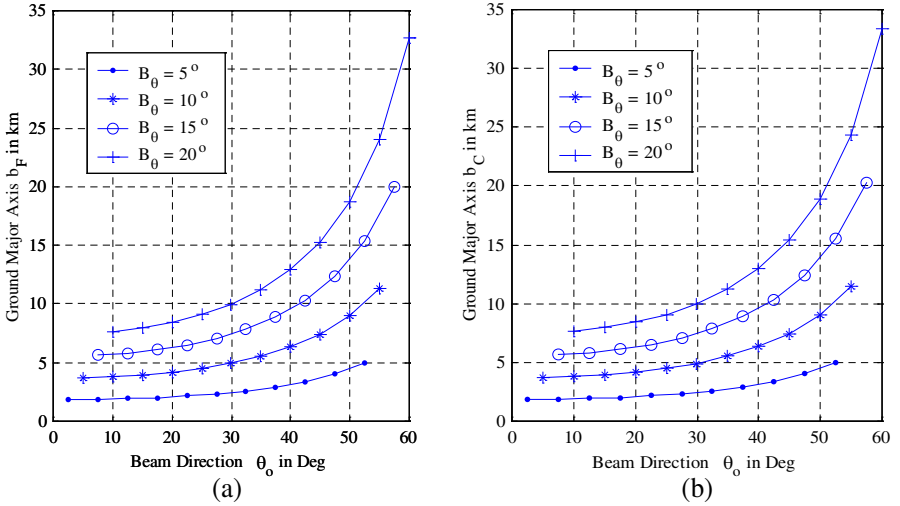
Figure 4. (a) b_F variation with beam direction at different beamwidths. (b) b_C variation with beam direction at different beamwidths.
