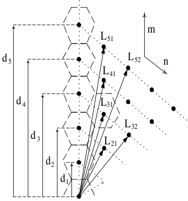
Figure 9. Central distance L_{mn} and radial distance d_m for some cells located in the first sector cell.
