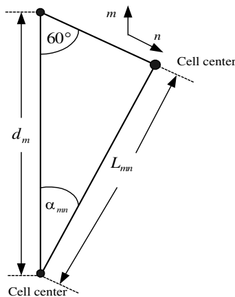
Figure 8. Coordinate system for cell location determination.
