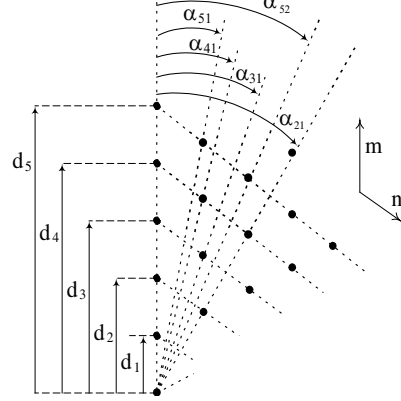
Figure 10. Central azimuth angle \alpha_{mn} for some cells located in the first sector.
