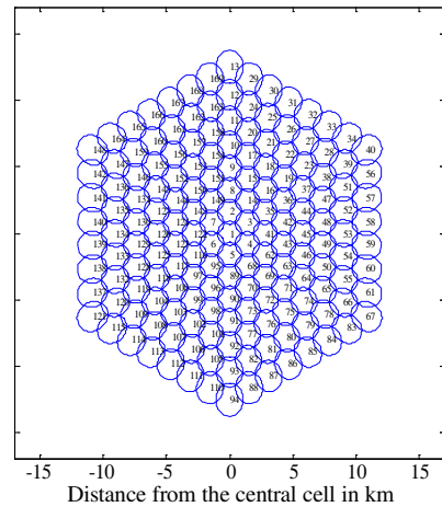
Figure 13. SP cellular layout constructed by 169 cell using spot-beam antennas of 5.0781^\circ beamwidth.
