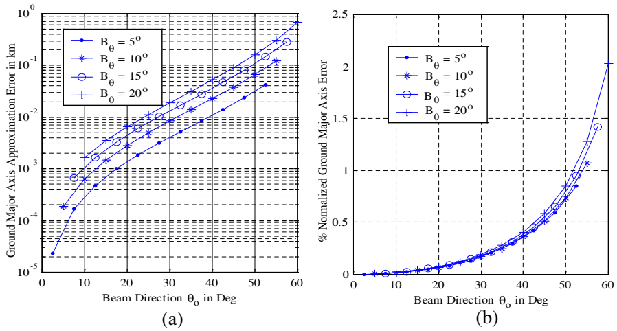
Figure 5. (a) Ground approximation error variation with beam direction at different beamwidths. (b) Relative error variation with beam direction at different beamwidths.
