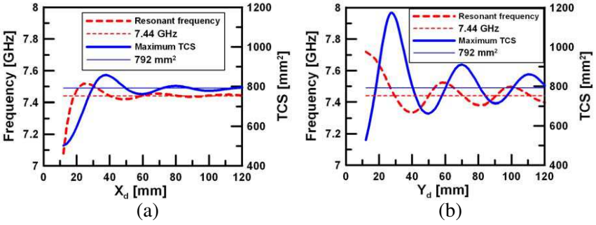
Figure 4. Resonant frequency and maximum TCS [MoM]: (a) Collinear case. (b) Parallel case.
