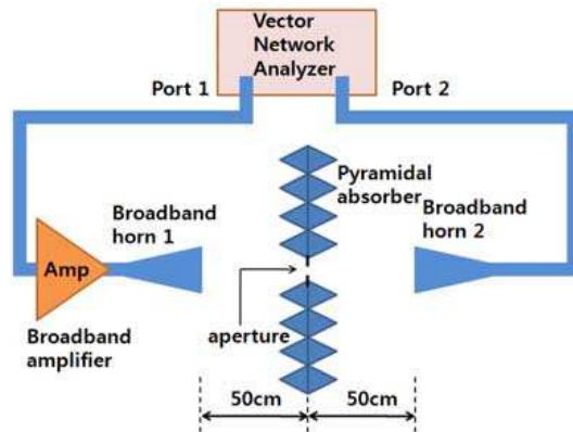
Figure 7. Experimental set-up for measurement.
