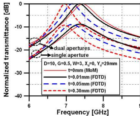
Figure 6. Normalized transmittance of a single aperture and parallel aperture pair ( Y_d = 29 mm) for t = 0 mm, 0.01 mm, 0.05 mm, and 0.30 mm [MoM and FDTD].
