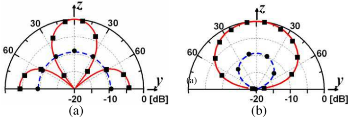
Figure 5. Radiation patterns at f = 7.44 GHz for the two parallel apertures having maximum TCS ( Y_d = 29 mm): (a) E -plane ( yz -plane). (b) H -plane ( xz -plane). t = 0 mm, D = 10 mm, W = 3 , and G = 0.5 mm. Dual aperture: Solid line (MoM), ■ (FDTD). Single aperture: Dashed line (MoM), ● (FDTD).
