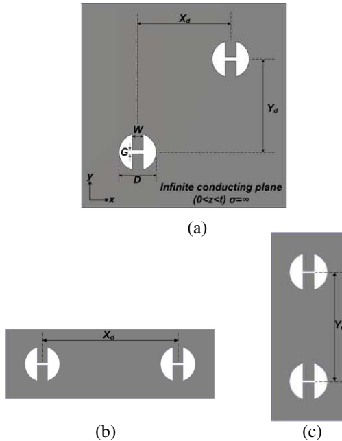
Figure 1. Geometry of a pair of ridge-loaded circular apertures in an infinite conducting plane: (a) Aperture pair in an arbitrary position in the plane. (b) Collinear case ( Y_d = 0 ). (c) Parallel case ( X_d = 0 ).
