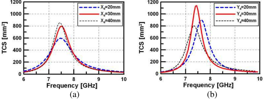
Figure 3. TCS characteristics [MoM]: (a) Collinear case. (b) Parallel case.
