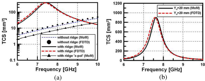
Figure 2. TCS variations: (a) Single aperture cases. (b) Dual apertures ( X_d = 0 mm, Y_d = 20 mm). t = 0 mm, D = 10 mm, W = 3 mm, and G = 0.5 mm.
