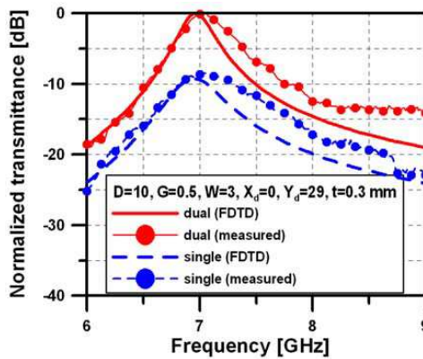
Figure 9. Comparison of the simulated and the measured transmittance characteristics of a single aperture and a parallel aperture pair ( Y_d = 29 mm) for t = 0.3 mm.
