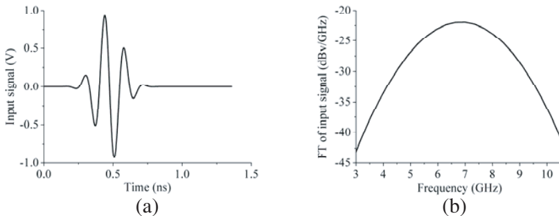
Figure 9. Time domain and frequency domain of the input signal. (a) The input signal. (b) Fourier transform of the input signal.
