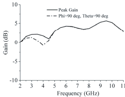
Figure 8. Measured peak gain and the gain in y direction of the antenna.
