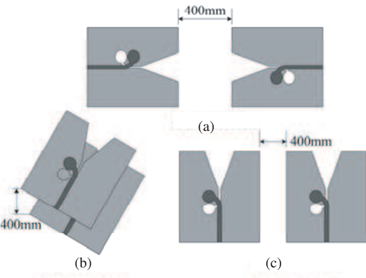
Figure 12. The communication link established of the antennas in different types: (a) Face to face. (b) Face to side. (c) Side to side.
