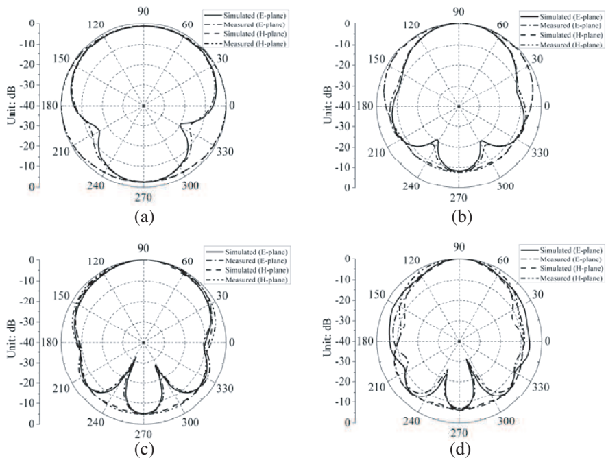
Figure 7. Simulated and measured radiation patterns of the proposed slot antenna in E -plane and H -plane at different frequencies. (a) 3.5 GHz. (b) 6 GHz. (c) 8 GHz. (d) 10 GHz.
