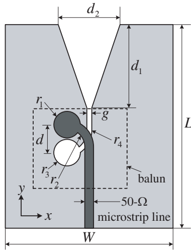
Figure 1. The configuration of the proposed antenna.
