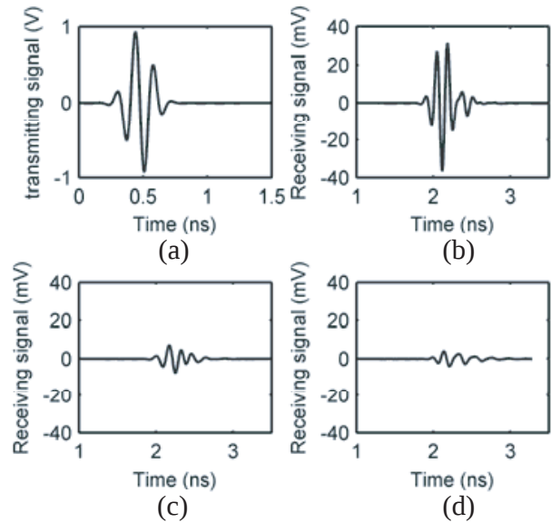
Figure 13. Receiving signals of the antennas in different types: (a) Input signal. (b) Face to face. (c) Face to side. (d) Side to side.
