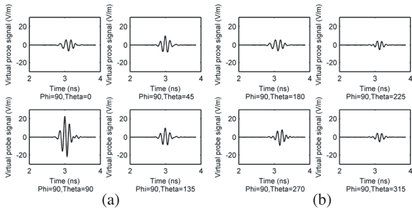
Figure 10. Virtual probe signals of the proposed antenna in different angles. (a) \varphi = 90^\circ , \theta = 0^\circ, 45^\circ, 90^\circ, 135^\circ . (b) \varphi = 90^\circ , \theta = 180^\circ, 225^\circ, 270^\circ, 315^\circ .
