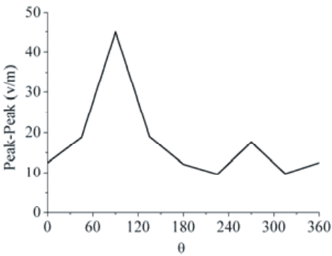
Figure 11. Peak-peak values of the virtual probe signals in different angles with \varphi = 90^\circ .
