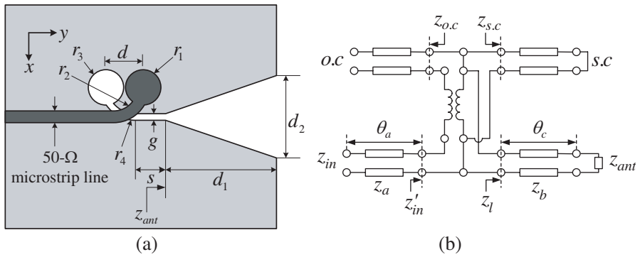
Figure 4. The proposed antenna: (a) The layout and (b) the equivalent circuit.
