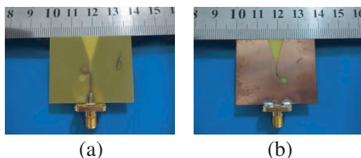
Figure 5. Photographs of the fabricated antenna. (a) The top side. (b) The bottom side.
