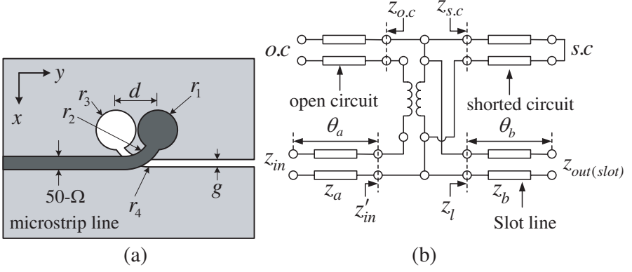
Figure 2. Microstrip to slotline transition line: (a) The layout and (b) the equivalent circuit.
