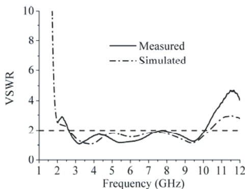
Figure 6. The simulated and measured responses of VSWR of the antenna.
