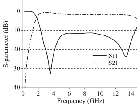
Figure 3. Simulated S -parameters of the microstrip to slot transition.
