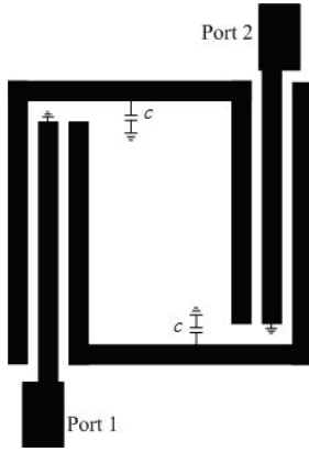
Figure 8. Structure of the proposed dual-band bandpass filter.
