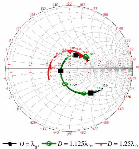
Figure 2. Impedance variation of FPA.
