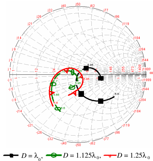
Figure 6. Impedance variation on finite ground of 9 \times 9 SPPA.
