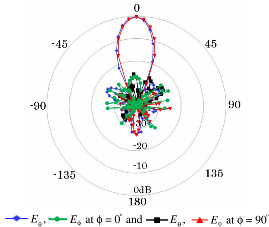
Figure 12. Measured radiation patterns of FPA ( D = 1.125\lambda_0 ) with 9 \times 9 SPPA antenna at 5.8 GHz.
