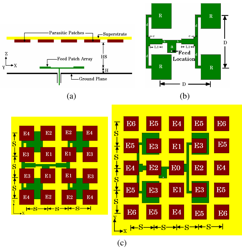
Figure 1. Geometry of proposed antenna structure. (a) Side view. (b) Top view of FPA. (c) 4 \times 4 and 5 \times 5 SPPA on a superstrate layer (top view).
