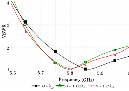
Figure 7. VSWR vs. frequency of 9 \times 9 SPPA.
