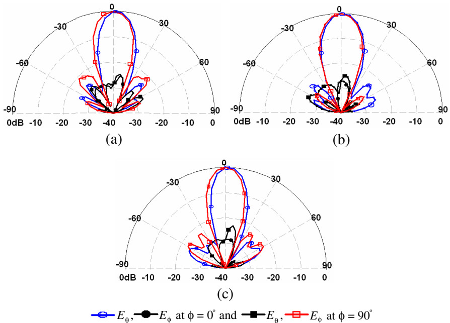
Figure 5. Radiation patterns of 9 \times 9 SPPA antenna at 5.8 GHz on infinite ground plane. (a) D = \lambda_0 . (b) D = 1.125\lambda_0 . (c) D = 1.25\lambda_0 .
