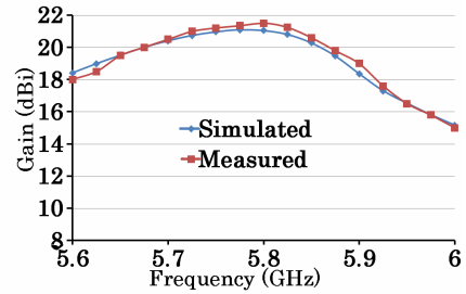
Figure 11. Gain vs. frequency of FPA ( D = 1.125\lambda_0 ) with 9 \times 9 SPPA.
