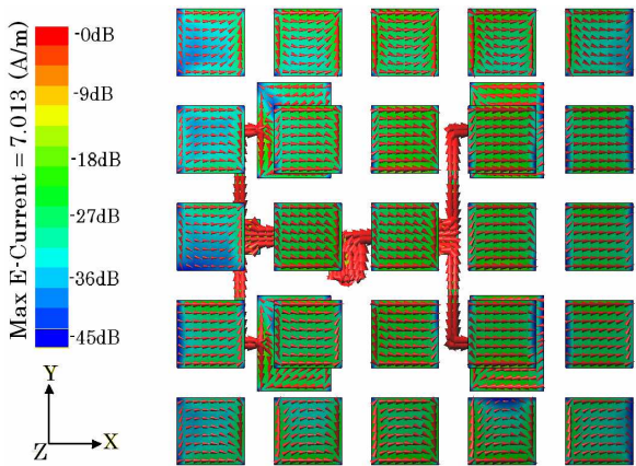
Figure 3. Current distribution of FPA ( D = 1.125\lambda_0 ) with 5 \times 5 SPPA at 5.8 GHz.
