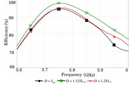
Figure 8. Antenna efficiency vs. frequency of 9 \times 9 SPPA on finite ground.
