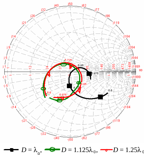
Figure 4. Impedance variation of FPAs with 9 \times 9 SPPA.
