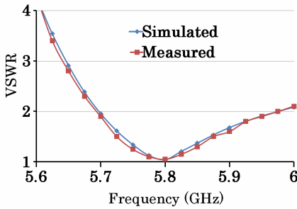
Figure 10. VSWR vs. frequency of FPA ( D = 1.125\lambda_0 ) with 9 \times 9 SPPA.
