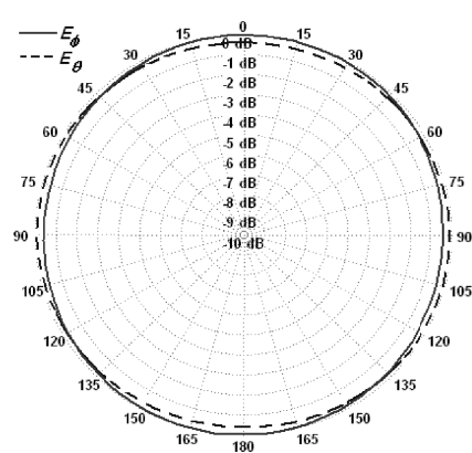
Figure 7. Azimuth radiation patterns; \theta = 120^\circ .
