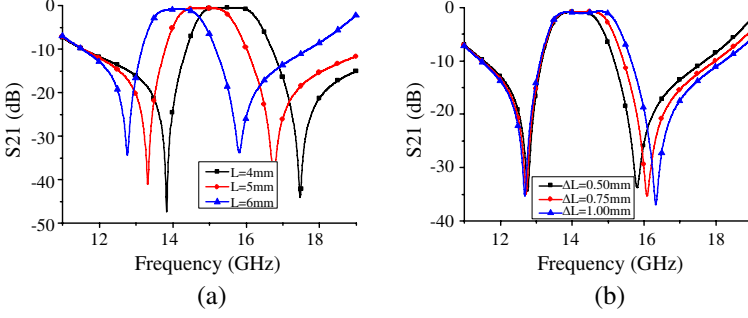
Figure 3. Simulated insertion loss of different slot length L and \Delta L for pure cross-slot SIW dualmode filter.
