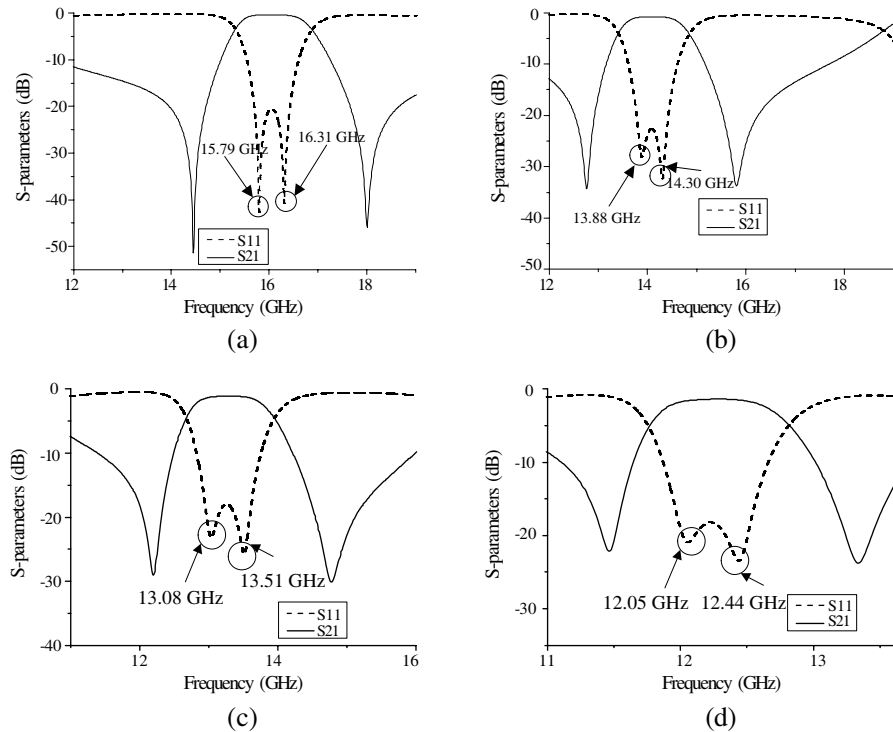
Figure 2. Simulated S parameters of original SIW dual-mode filter and the proposed family of filters, (a) original filter, (b) pure cross-slot, (c) T-shaped loaded cross-slot, (d) H-shaped loaded.
