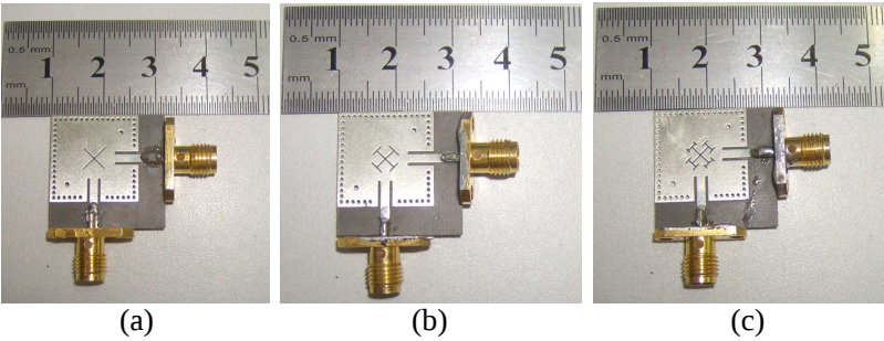
Figure 6. Photograph of fabricated miniaturized SIW dual-mode filters with (a) pure cross-slot, (b) T-shaped loaded cross-slot, (c) H-shaped loaded cross-slot.
