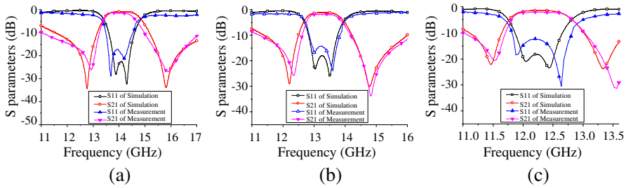
Figure 7. Simulated and measured frequency responses of the proposed family of SIW dual-mode filters with (a) pure cross-slot, (b) T-shaped loaded cross-slot, (c) H-shaped loaded cross-slot.
