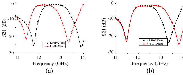
Figure 5. Simulated insertion loss of different whole slot length L_{wH} and difference between the two H-shaped stubs \Delta L_H for H-shaped loaded cross-slot SIW dual-mode filter.
