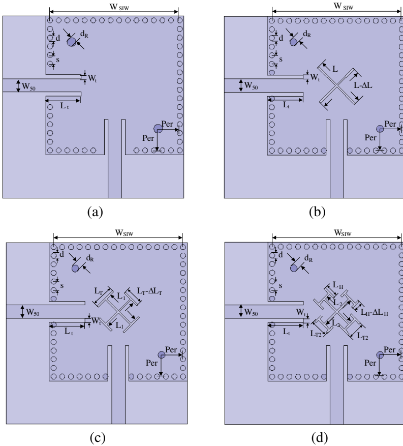
Figure 1. Configuration of original SIW dual-mode filter and the proposed family of filters, (a) original filter, (b) pure cross-slot, (c) T-shaped loaded cross-slot, (d) H-shaped loaded cross-slot.
