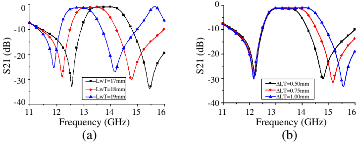
Figure 4. Simulated insertion loss of different whole slot length L_{wT} and difference between the two T-shaped stubs \Delta L_T for T-shaped loaded cross-slot SIW dual-mode filter.
