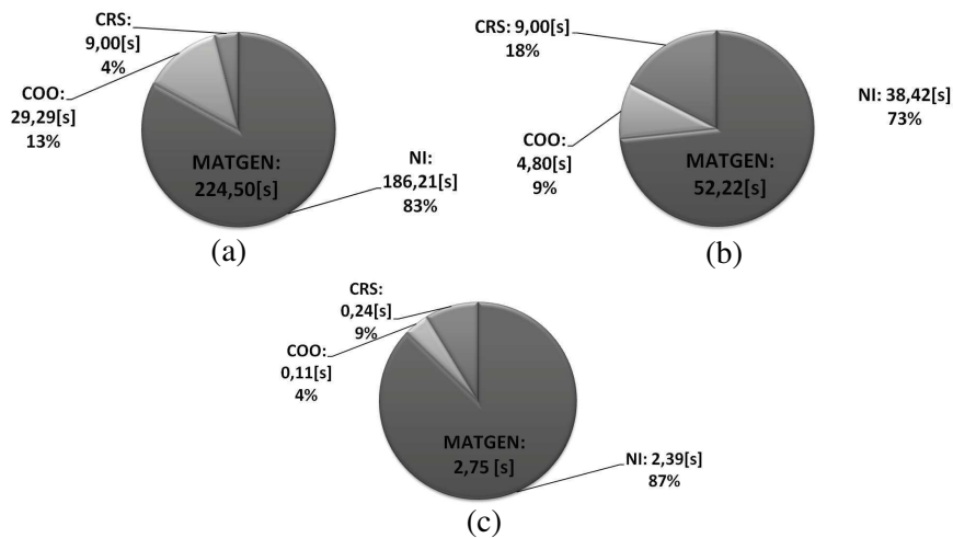
Figure 3. The finite matrix generation (TEST2) — time share required for the numerical integration (NI), matrix assembly into the COO format (COO) and conversion from the COO to CRS format (CRS). Test platforms GPU: (Tesla C2075) and CPU (2x twelve-core Opterons 6174). (a) Opteron — 1 thread. (b) Opteron — 24 thread. (c) Tesla C2075.
