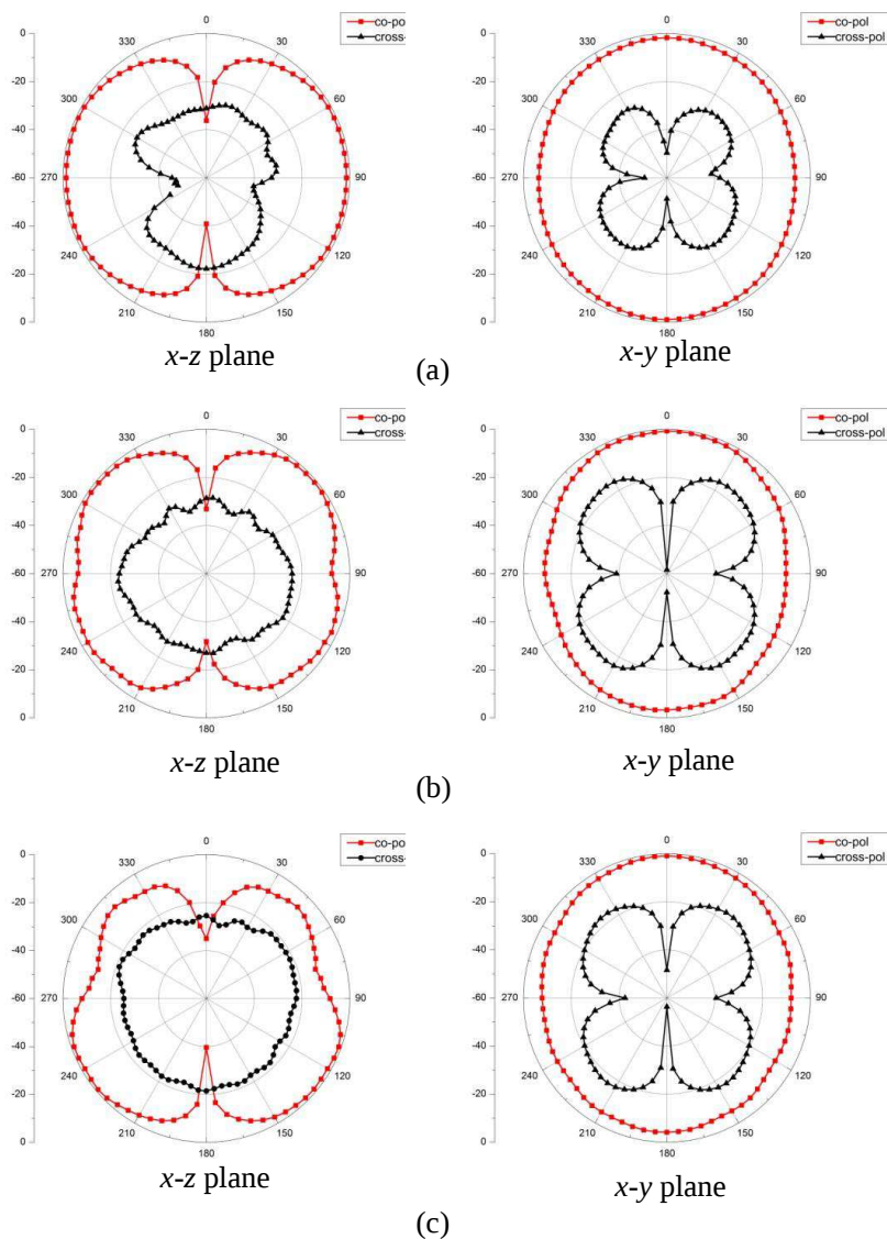
Figure 7. Radiation patterns at (a) 3.5 GHz, (b) 5.3 GHz, (c) 5.9 GHz.
