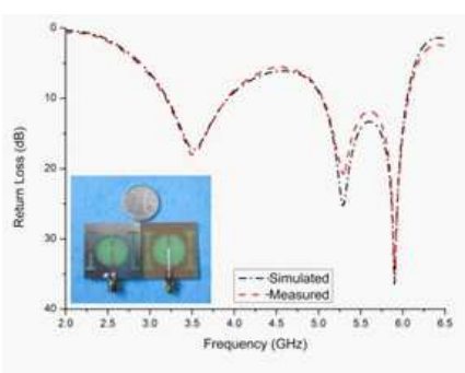
Figure 5. Simulated and Measured return losses of the antenna.
