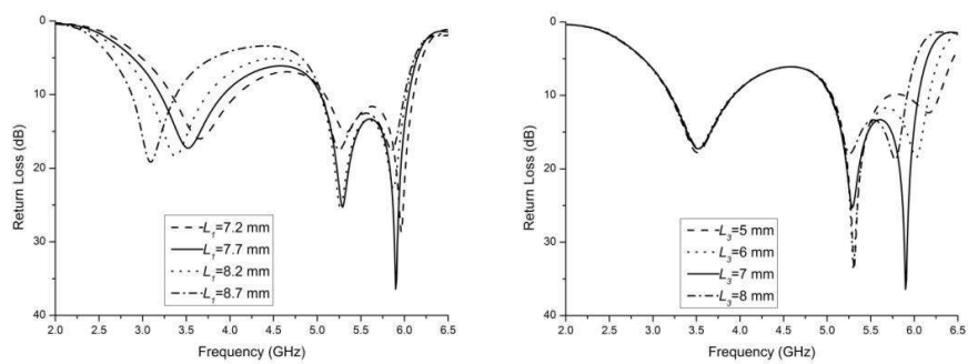
Figure 3. Effect of varying ground plane parameters on the antenna performance. (a) Length of the straight strip ( L_1 ). (b) Length of the T-shaped slot ( L_3 ).
