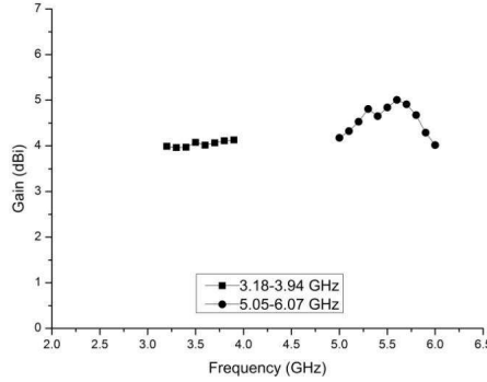
Figure 8. Gain of the proposed antenna.
