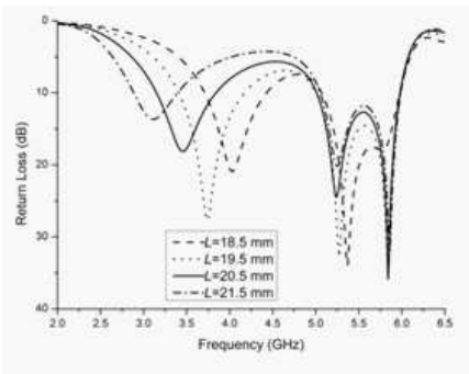
Figure 4. Simulated return loss for different values of L .
