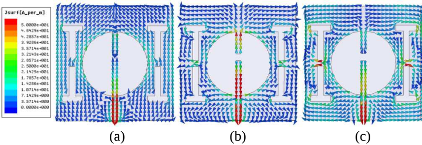
Figure 6. Simulated current distribution at (a) 3.5 GHz, (b) 5.3 GHz, (c) 5.9 GHz.
