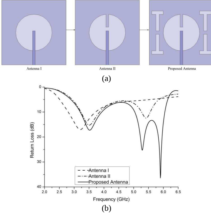
Figure 2. (a) Design evolution of the proposed antenna and (b) its corresponding simulated return loss results.
