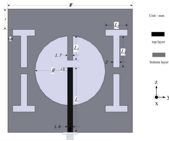
Figure 1. Antenna configuration and detailed dimensions ( W = 39 mm, R = 11 mm, L = 20.5 mm, L_1 = 7.7 mm, L_2 = 7 mm, L_3 = 10 mm, h = 1 mm, g = 1.5 mm, t = 6.5 mm).
