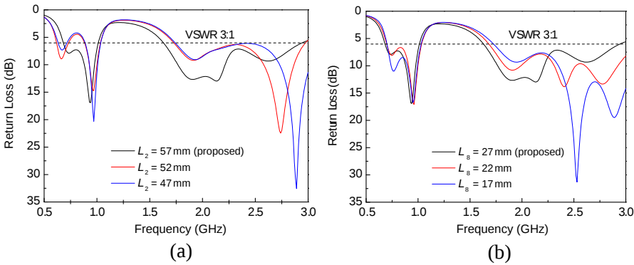
Figure 5. Parametric study for the proposed antenna. (a) strip L_2 , (b) strip L_8 .
