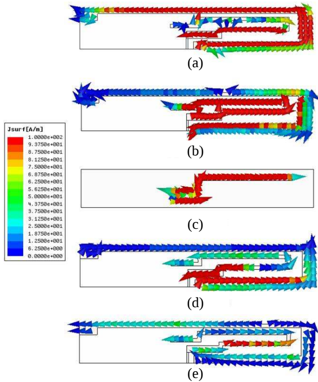
Figure 2. Simulated surface current distributions for the proposed antenna. (a) 720 MHz, (b) 940 MHz, (c) 1900 MHz, (d) 2120 MHz, (e) 2600 MHz.
