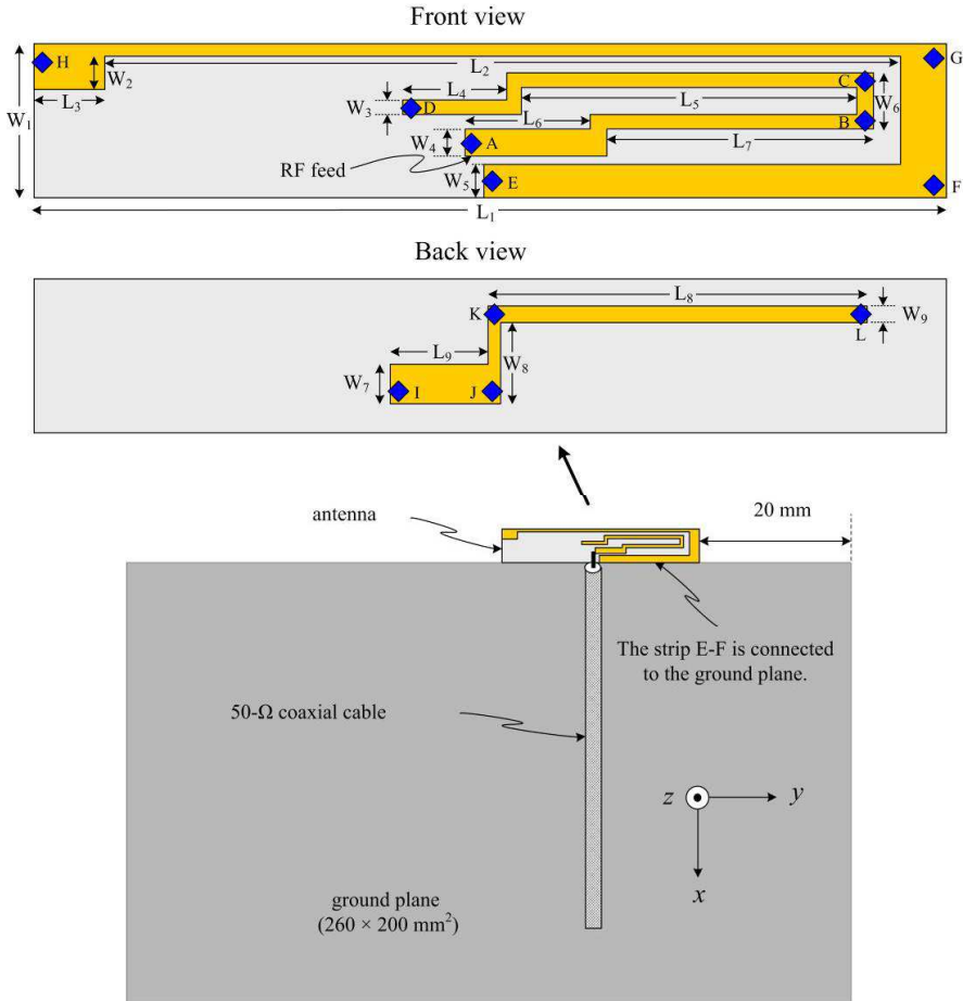
Figure 1. Design structure of the proposed eight-band LTE/WWAN monopole antenna. ( L_1 = 65 mm, L_2 = 57 mm, L_3 = 5 mm, L_4 = 7.5 mm, L_5 = 24 mm, L_6 = 9 mm, L_7 = 19 mm, L_8 = 27 mm, L_9 = 7 mm, W_1 = 11 mm, W_2 = 2 mm, W_3 = 1 mm, W_4 = 2 mm, W_5 = 2 mm, W_6 = 4 mm, W_7 = 2.8 mm and W_8 = 5.8 mm).
