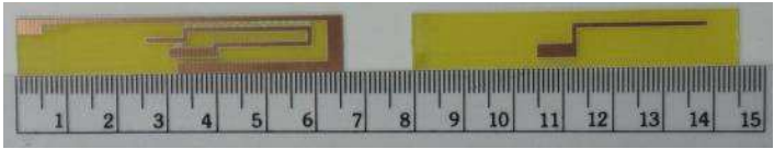
Figure 3. Fabricated prototype of the proposed antenna.
