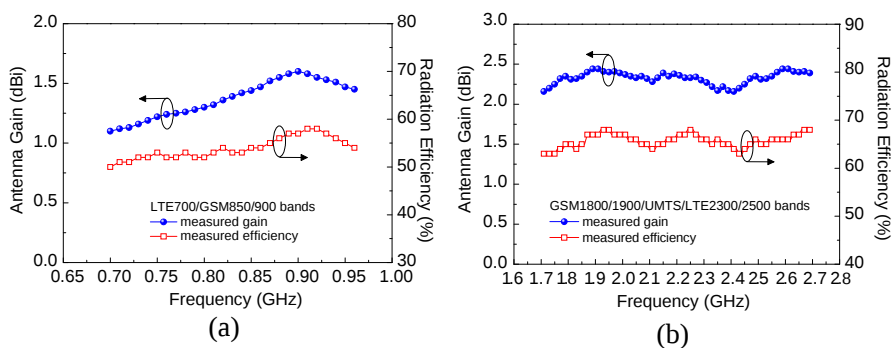
Figure 7. Measured peak gain and radiation efficiency of the proposed antenna. (a) LTE700/GSM850/900 bands, (b) GSM1800/1900/UMTS/LTE2300/2500 bands.
