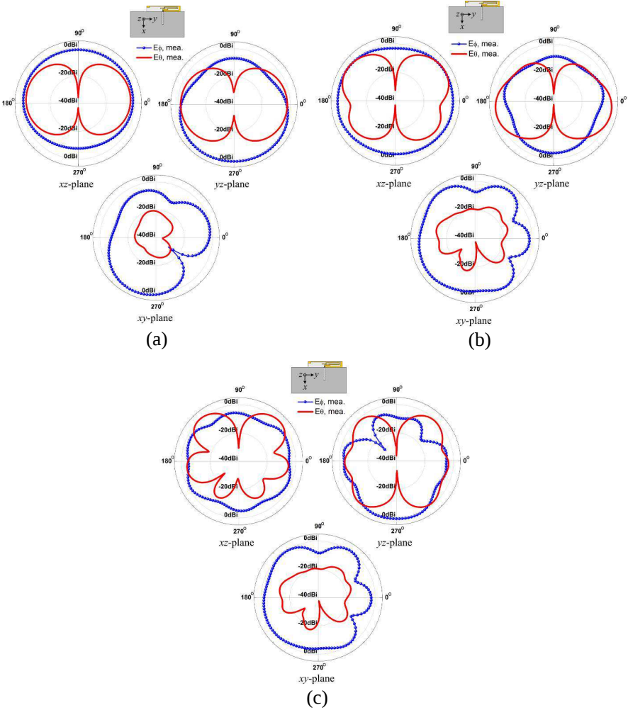
Figure 6. Measured radiation patterns of the proposed antenna. (a) 860 MHz, (b) 1800 MHz, (c) 2600 MHz.
