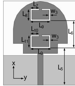
Figure 4. Configuration of the band-rejected UWB antenna for lower WLAN band.
