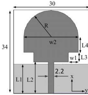
Figure 1. Geometry of the proposed UWB antenna (Unit: mm)
