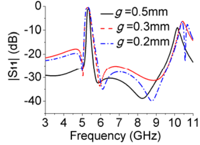
Figure 14. |S_{11}| for different g .
