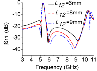
Figure 16. |S_{11}| for different L_{12} .
