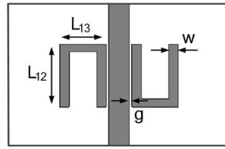
Figure 11. Geometry of the proposed band-stop filter.
