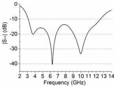
Figure 3. Return loss of the UWB antenna without band-rejected structure.
