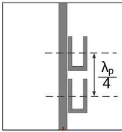
Figure 10. Traditional structure of two order band-stop filter.
