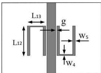
Figure 17. Two order band-stop filter with SIR structure.
