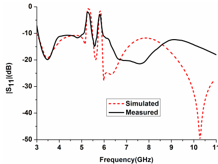
Figure 20. The simulated and measured return losses of the proposed antenna.
