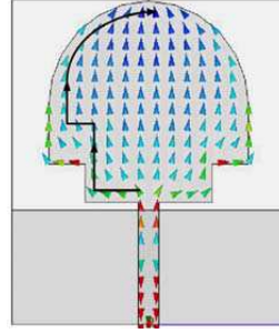
Figure 2. The current distributions at 3.1 GHz.
