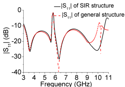
Figure 18. Simulated |S_{11}| with UR and SIR structure.
