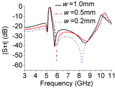
Figure 15. |S_{11}| for different w .
