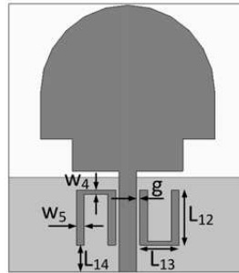
Figure 9. Configuration of the band-rejected UWB antenna for upper WLAN band.
