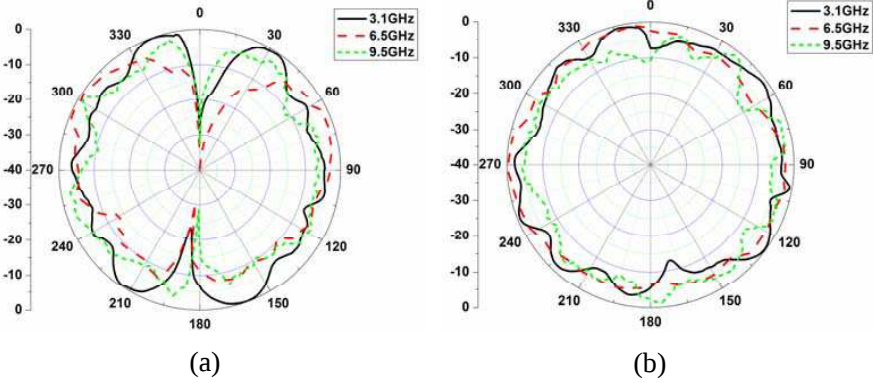
Figure 21. Measured radiation patterns of the proposed antenna at 3.1, 6.5 and 9.5 GHz. (a) E -plane ( xy ). (b) H -plane ( yz ).
