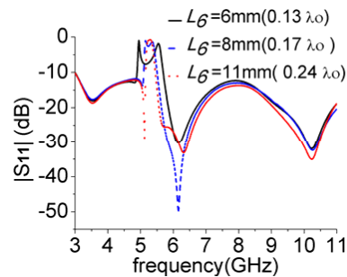
Figure 6. Simulated |S_{11}| with different L_6 .
