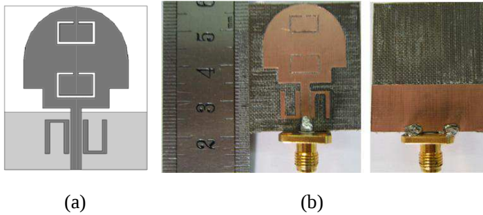
Figure 19. The geometry of the proposed antenna. (a) Schematic diagram. (b) Fabricated sample of top and bottom view.
