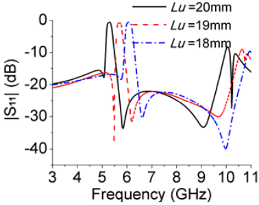
Figure 13. |S_{11}| for different L_u .
