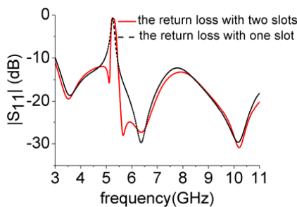
Figure 5. Simulated |S_{11}| with one and two slits.
