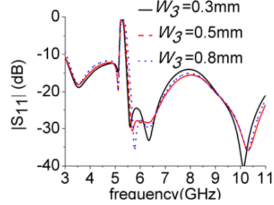
Figure 7. |S_{11}| with different L_9 . Figure 8. |S_{11}| with different w_3 .
