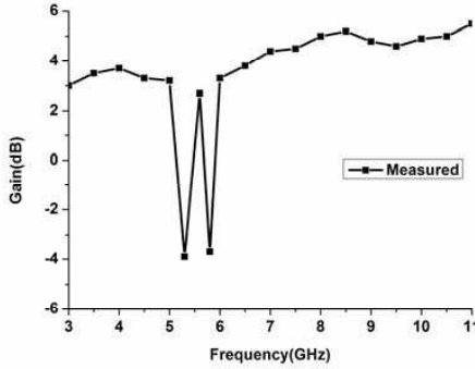
Figure 22. Measured Gain of proposed antenna.
