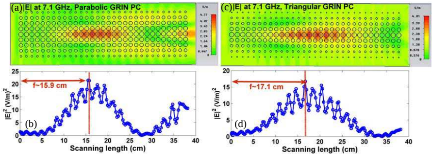
Figure 2. (a) and (b) show the focusing and the corresponding scanning plot of the parabolic GRIN medium. (c) and (d) show the focusing and the scanning plot for the triangular index GRIN medium. Both use a gradient coefficient of \alpha = 0.1172a^{-1} at 7.1 GHz.
