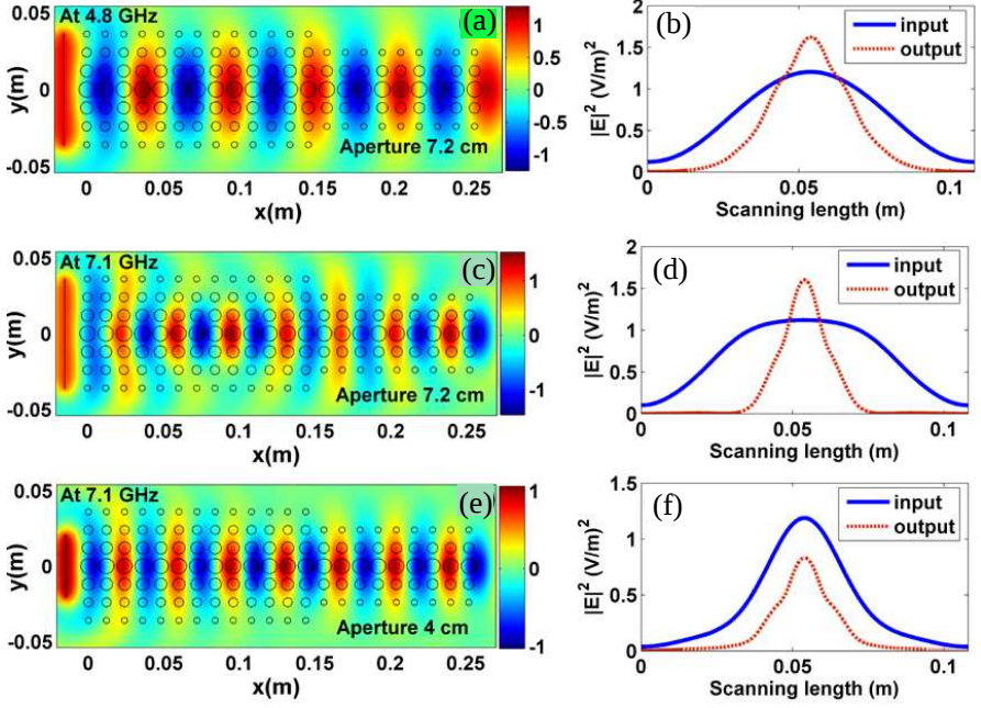
Figure 4. (a) E_z field map at 4.8 GHz for the finite aperture size of 7.2 cm and (b) shows the corresponding electric field intensity profiles at the input ( i/p )/output ( o/p ) planes. (c) E_z field map at 7.1 GHz for the aperture size of 7.2 cm and (d) shows the corresponding |E|^2 profiles of the i/p and o/p beams. (e) E_z field map at 7.1 GHz for the aperture size of 4 cm and (f) shows the corresponding |E|^2 profiles of the i/p and o/p beams.
