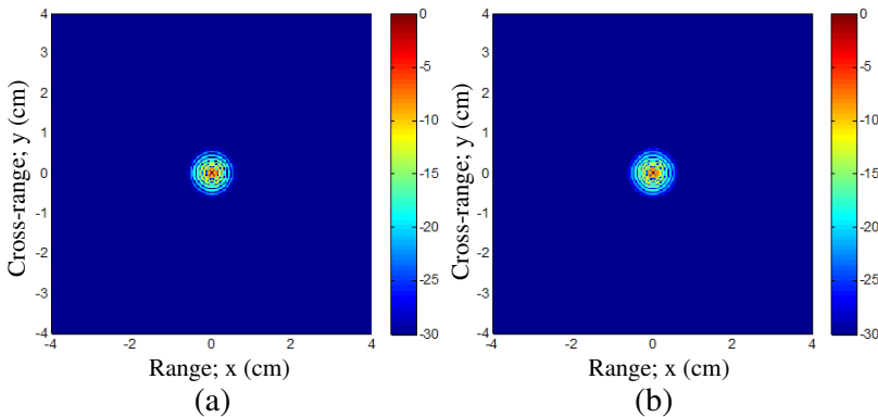
Figure 2. PSF images for an angular span of 0^\circ \sim 360^\circ with 361 sampling points and a frequency span of 80 \sim 100 \text{ GHz} with 256 sampling points: (a) Focusing operator, (b) back-projection based imaging.
