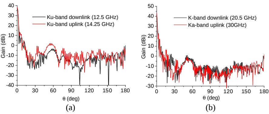
Figure 7. Simulated gain patterns of the 650mm diameter 7-layer LLA (solution A), (a) Ku-band downlink/uplink, (b) K-band downlink and Ka-band uplink.
