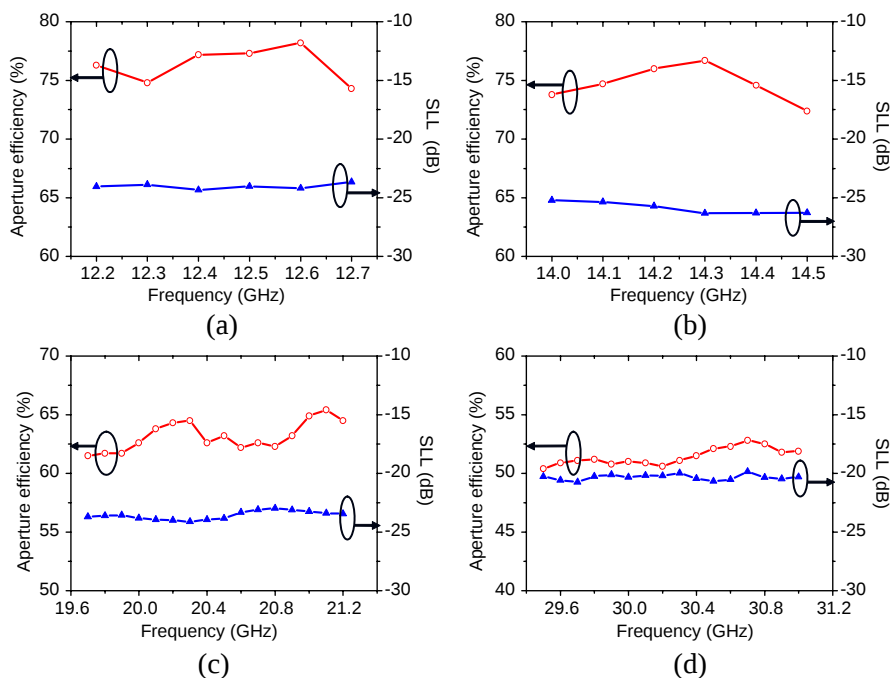
Figure 8. Frequency dependence of the 7-layer optimized LLA. (a) Ku-band downlink. (b) Ku-band uplink. (c) K-band downlink. (d) Ka-band uplink.
