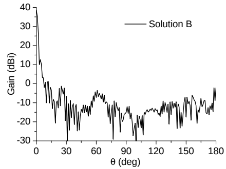
Figure 10. The MOEA/D optimized radiation pattern of the 5-layer 30\lambda diameter LLA at Ku-band downlink (solution B).
