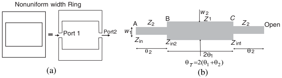
Figure 3. (a) Non-uniform width ring geometry and its equivalent two-port network. (b) Transmission line section of (a).
