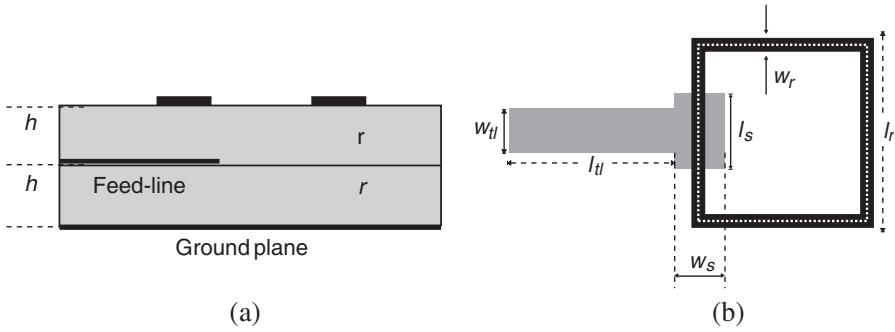
Figure 1. Geometry of the ring antenna.
