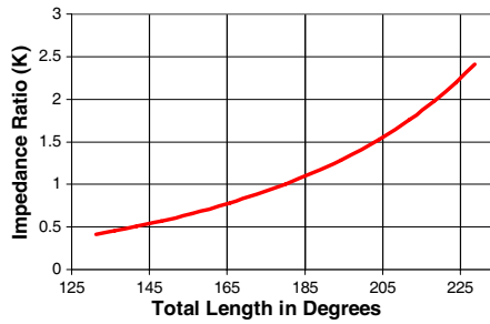
Figure 4. Resonant condition of the stepped impedance resonator.
