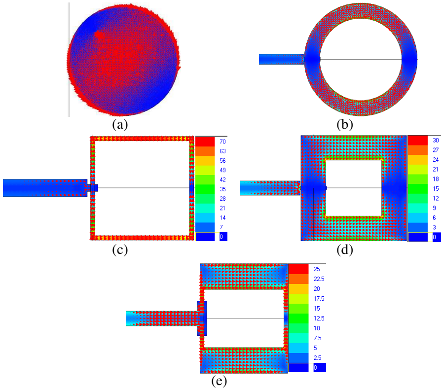
Figure 6. Simulated current distribution at the primary resonance of various antennas. (a) Patch antenna at resonance. (b) Narrow annular ring at resonance. (c) Narrow square ring at resonance. (d) Wide uniform ring at resonance. (e) Non-uniform width ring at resonance.
