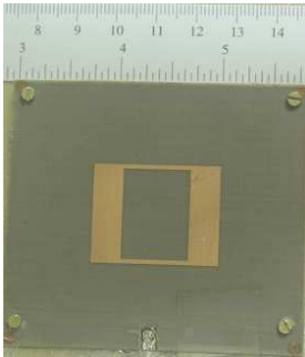
Figure 7. Photograph of a fabricated non-uniform width square ring antenna.
