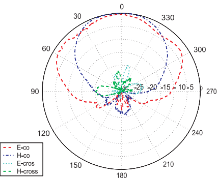
Figure 9. Measured radiation patterns of the non-uniform width ring antenna at 3.151 GHz.
