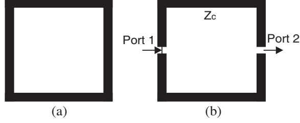
Figure 2. (a) An isolated ring geometry and (b) its equivalent two-port network.
