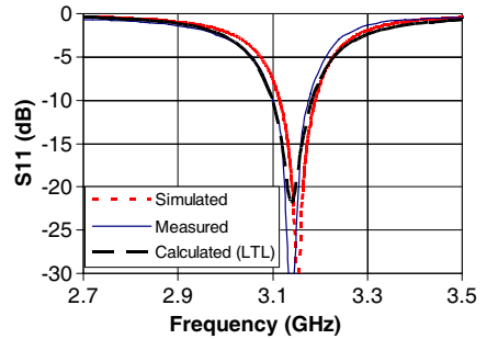
Figure 8. S_{11} characteristics of fabricated non-uniform width square ring antenna.
