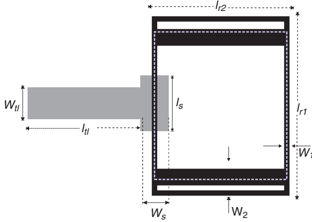
Figure 5. Geometry of the non-uniform width ring antenna.
