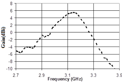
Figure 10. Measured gain of the antenna.
