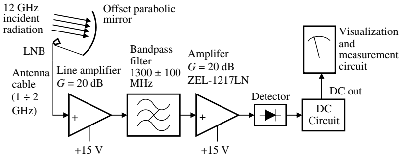
Figure 2. Block diagram of the receiving system.
