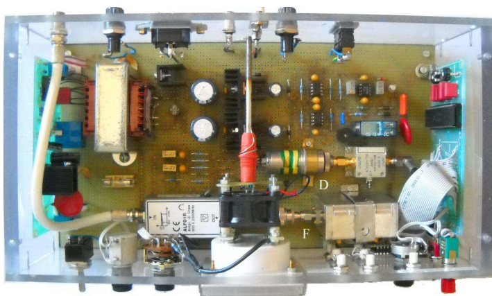
Figure 8. Implementation of the radio telescope. F: bandpass filter; D: detector.
