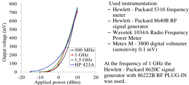
Figure 6. Measures on the detector circuit in semi-logarithmic scale. The commercial detector HP423@1.5 GHz was measured at only one frequency (1.5 GHz).
