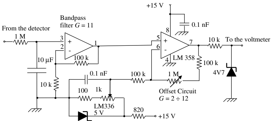
Figure 7. DC circuit.
