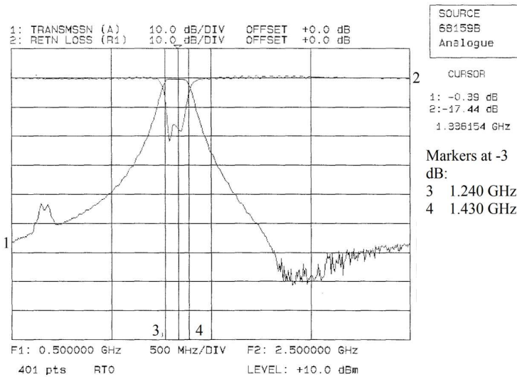
Figure 4. Measurements of the IF filter using a vector network analyzer HP 8722 D. The measures displayed confirm clearly the predictions made in the theoretical calculation. The insertion loss of only 0.39 dB and the return loss, which is on average 20 dB in the band of operation, reflect a very good performance.
