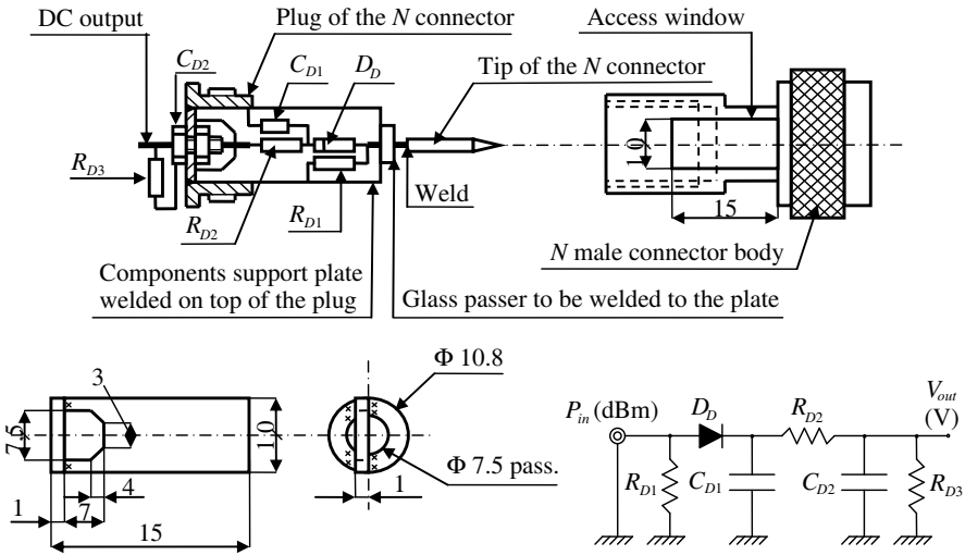
Components support plate. Material: Brass \neq 1. Tin solders.
