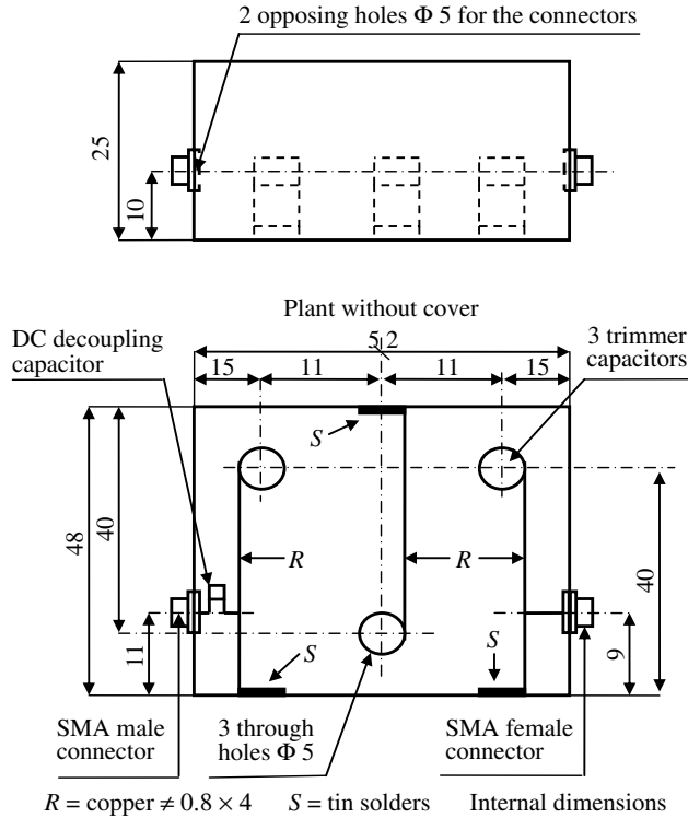
Figure 3. Drawing of the bandpass filter.
