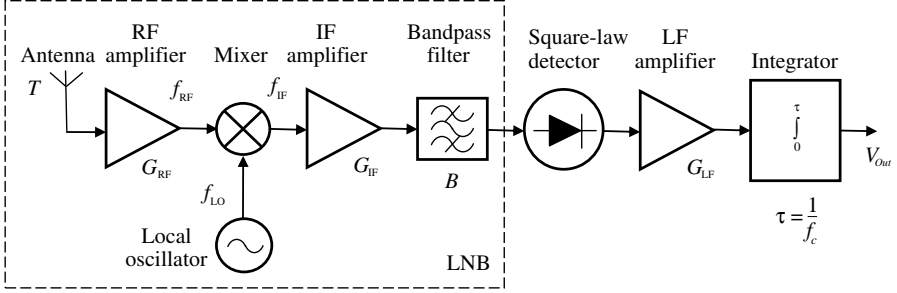
Figure 1. Block diagram of a “total power” radio telescope. We have indicated with: T the temperature of the antenna, G_{\text{RF}} the gain of the Radio Frequency (RF) amplifier, f_{\text{RF}} the frequency of the RF signal, f_{\text{LO}} the frequency of the local oscillator, f_{\text{IF}} the frequency of the Intermediate Frequency (IF) signal, G_{\text{IF}} the gain of the IF amplifier, B the bandwidth of the bandpass filter, G_{\text{LF}} the gain of the Low Frequency (LF) amplifier, \tau the time constant of the integrator.
