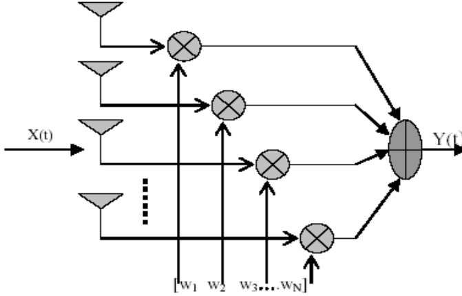
Figure 1. Narrow band antenna array with a complex weight.
