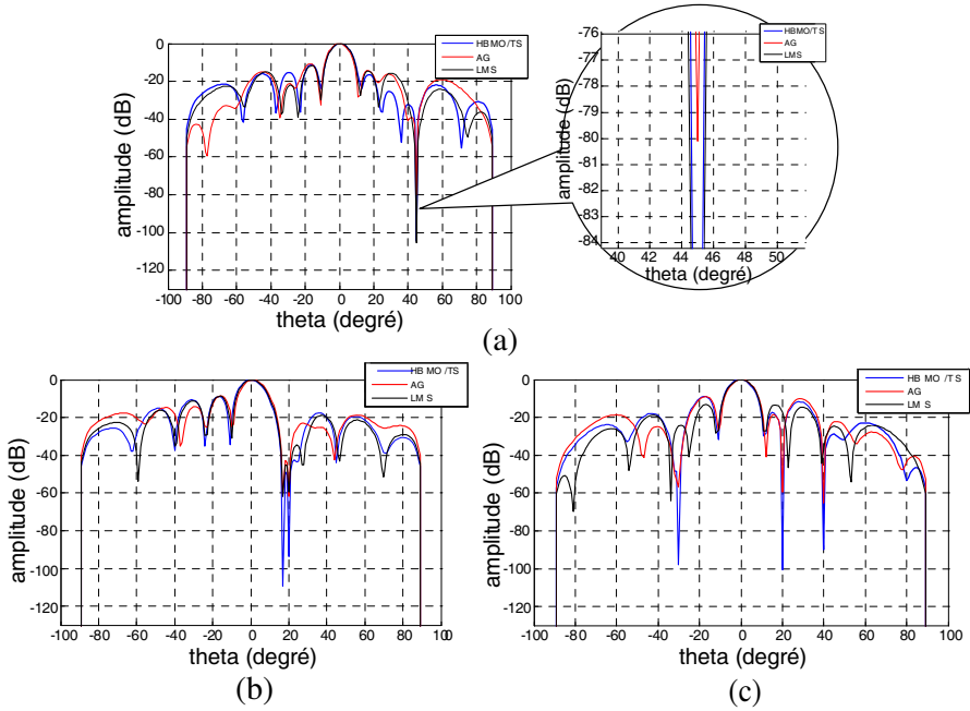
Figure 3. Interferences rejections: (a) interference rejection at 45^\circ , (b) two very close interferences rejections ( 17^\circ and 20^\circ ), (c) several interferences rejections (at -30^\circ , 20^\circ and 40^\circ ).
