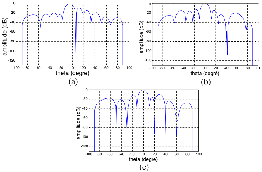
Figure 2. Interferences rejections by HBMO/TS: (a) interference rejection in the direction of the main lobe at 6^\circ , (b) two very close interferences rejections at 40^\circ and 42^\circ , (c) the case of several interferences rejections (interferences at -50^\circ , -30^\circ , 20^\circ , 40^\circ , 60^\circ ).
