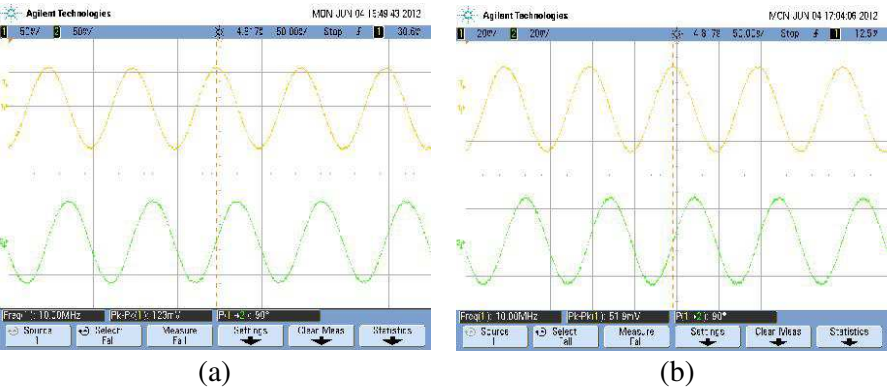
Figure 4. Calibration tone — time domain. (a) Proposed RWS, (b) Agilent N8241A AWG.
