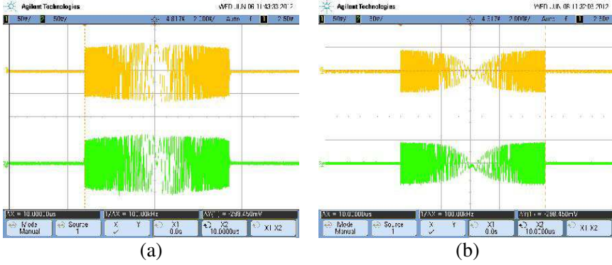
Figure 7. LFM waveform — time domain. (a) Proposed RWS, (b) Agilent N8241A AWG.
