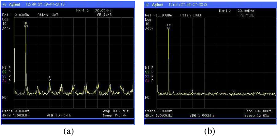
Figure 6. Calibration tone — broadband spurious harmonics. (a) Proposed RWS, (b) Agilent N8241A AWG.
