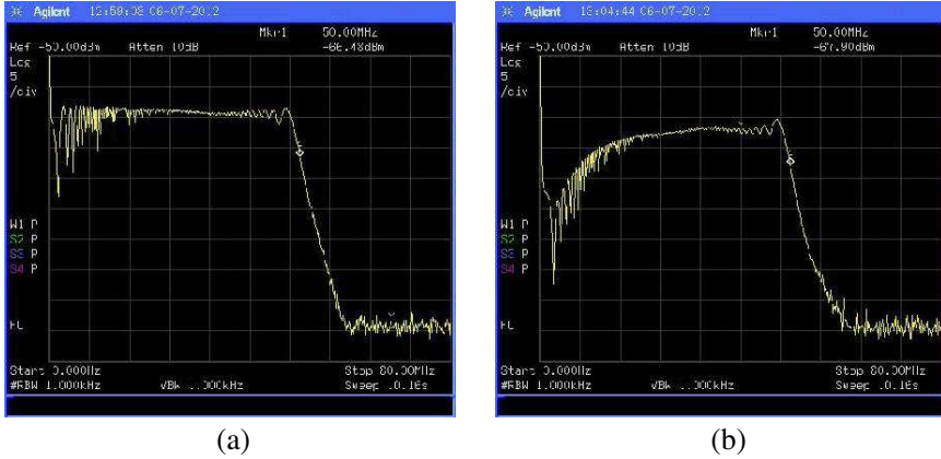
Figure 8. LFM waveform — frequency domain. (a) Proposed RWS, (b) Agilent N8241A AWG.
