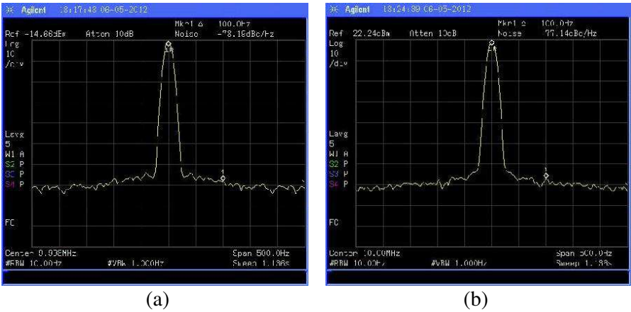
Figure 5. Calibration tone — phase noise. (a) Proposed RWS, (b) Agilent N8241A AWG.
