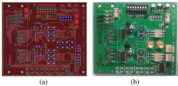
Figure 2. (a) HS-PCB layout design for HS-DAC board, (b) HS-DAC board
