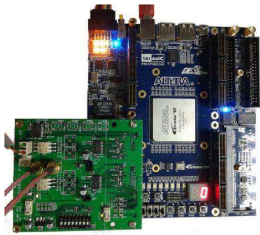
Figure 3. Altera DE3 development board and custom made HS-DAC board.
