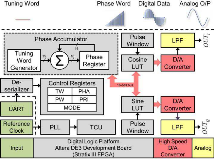
Figure 1. Proposed waveform synthesizer core.
