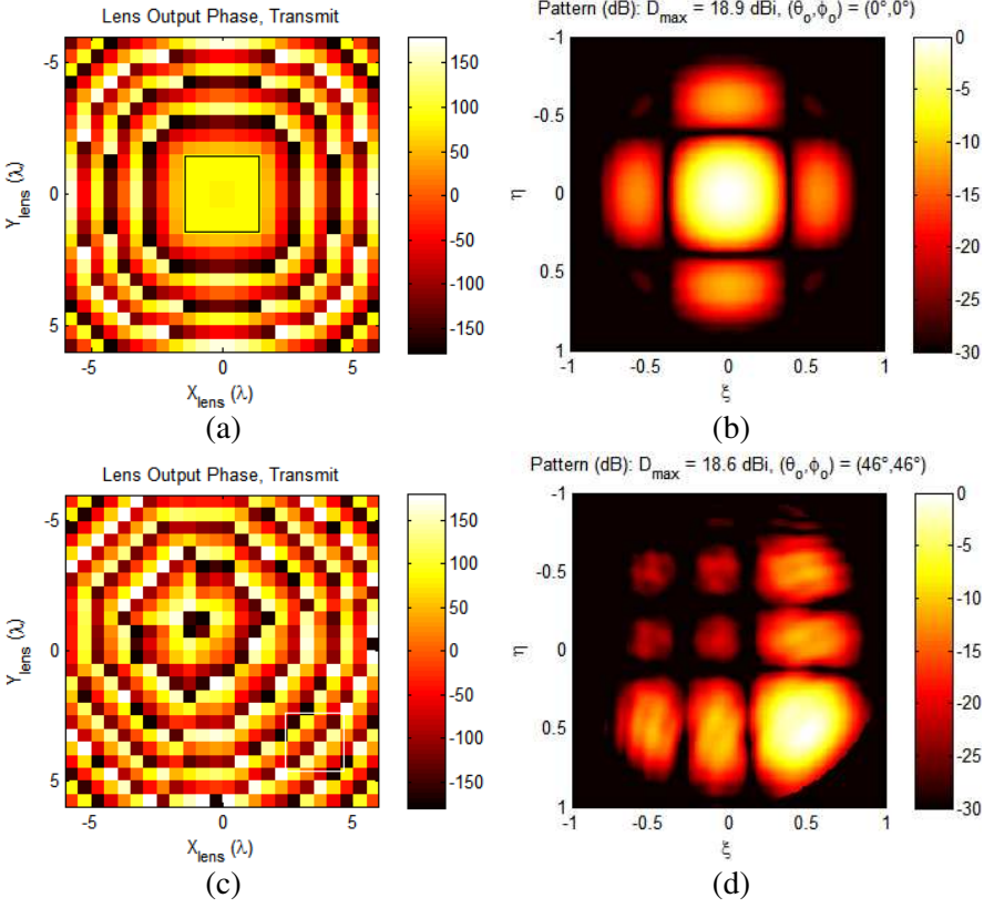
Figure 8. Simulation results for the LEPA with \varphi -focused LA: (a) LA output phase and (b) radiation pattern for boresight, (c) LA output phase and (d) radiation pattern for x_s = y_s = -28.7\lambda , z_s = -18.3\lambda .
