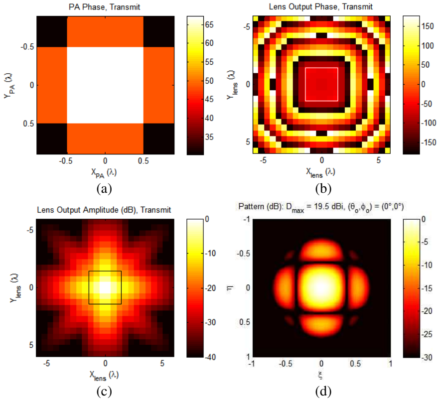
Figure 6. Simulation results for LEPA with modified lens set for boresight radiation: (a) PA phase profile, (b) LA output phase, (c) LA output amplitude, and (d) radiation pattern. The “lit region” is marked by square in (b) and (c).
