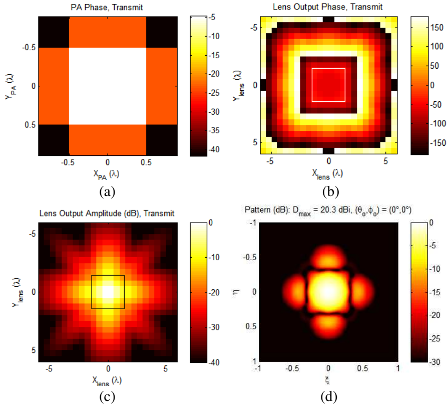
Figure 2. Simulation results for LEPA with standard LA, set for boresight radiation: (a) PA phase profile, (b) LA output phase, (c) LA output amplitude, and (d) radiation pattern. The “lit region” is marked by the squares in (b) and (c).
