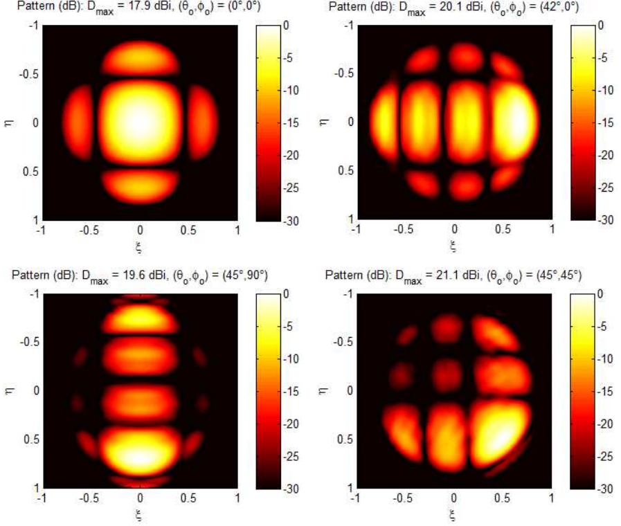
Figure 9. Simulation radiation pattern and peak directivity for a 60 GHz LEPA with L_1 = 9 mm, L_2 = 60 mm, G = 5 mm, and F = 23 mm for various scan angles.
