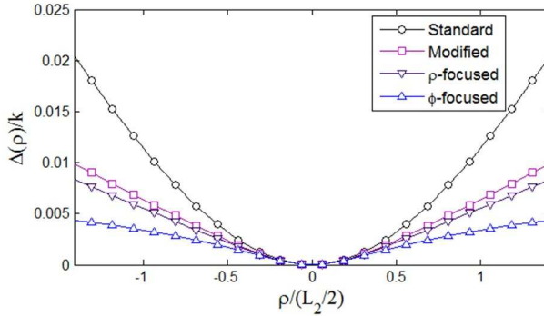
Figure 5. Phase delay profile for various lens designs.
