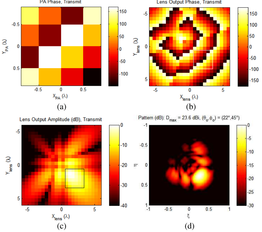
Figure 3. The LEPA system of Fig. 2 resimulated with the virtual source moved to x_s = y_s = -4.8\lambda , z_s = -6.8\lambda .
