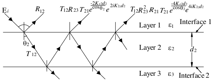
Figure 1. A series of multiple reflections from the geometric optics in a lossy three-layer model.
