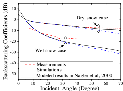
Figure 4. Comparison of simulated results with measurements at 5.3 GHz, VV-polarization.
