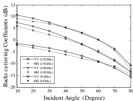
Figure 3. Effect of signal frequency variation on snow backscattering coefficients.
