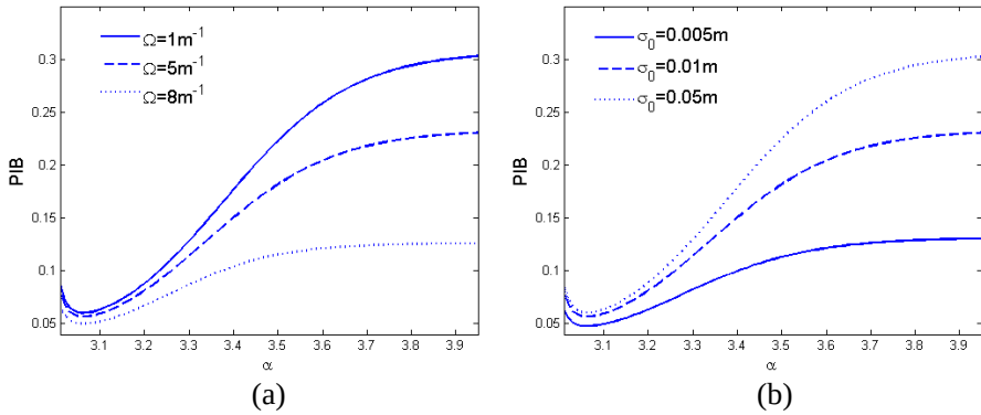
Figure 5. Dependence of PIB on \alpha .
