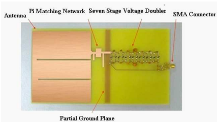
Figure 16. Integrated assembled PCB of RF energy harvesting system for GM-900.
