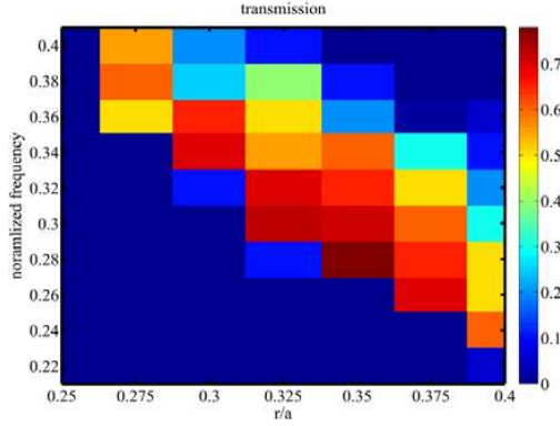
Figure 3. Transmittance contour plots for Normalized frequency a/\lambda versus different ratio of r/a in rod-type hexagonal PhC for a fixed incident angle, \theta_i = 0^\circ .
