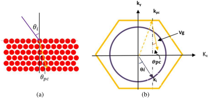
Figure 1. (a) Geometry showing the creation of incident and transmitted light at the boundary of a homogenous dielectric and a PhC media according to snell law, (b) the equifrequency contour of two homogeneous isotropic dielectrics and a PhC.
