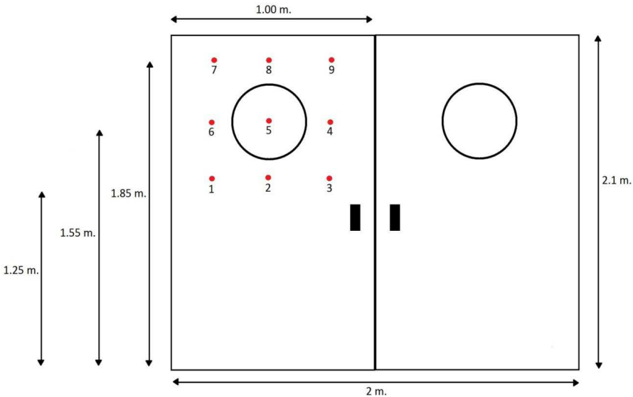
Figure 1. Metallic door with two porthole windows.
