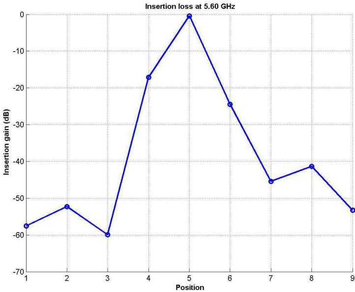
Figure 2. Insertion gain with horizontal polarization using two antennas with a gain of 19 dB.
