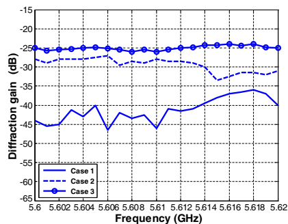
Figure 10. Diffraction gain for the vertical polarization.
