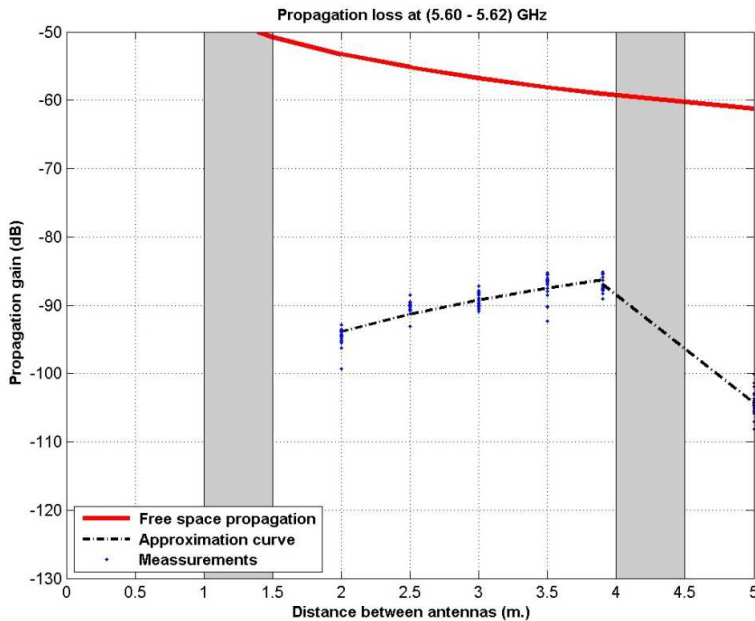
Figure 13. Propagation loss due to the second diffraction scenario with horizontal polarization and antenna gain of 19 dB at both transmitting and receiving sides.
