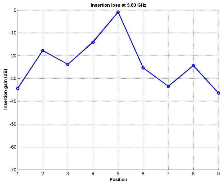
Figure 5. Insertion gain with vertical polarization using two antennas with a gain of 11 and 8 dB respectively.
