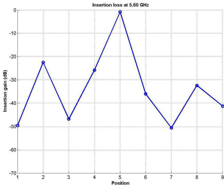
Figure 3. Insertion gain with vertical polarization using two antennas with a gain of 19 dB.
