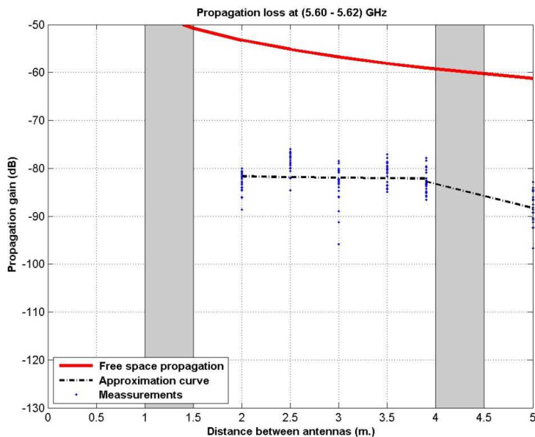
Figure 14. Propagation loss due to the second diffraction scenario with vertical polarization using a transmitting antenna with a gain of 11 dB and a receiving one with a gain of 8 dB.
