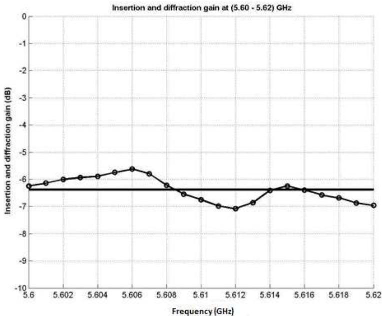
Figure 6. Wall insertion gain with horizontal polarization.
