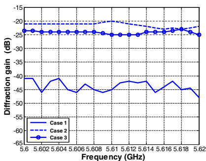
Figure 9. Diffraction gain for the horizontal polarization.
