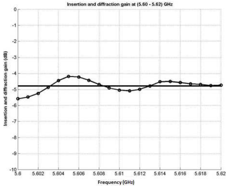
Figure 7. Wall insertion gain with vertical polarization.
