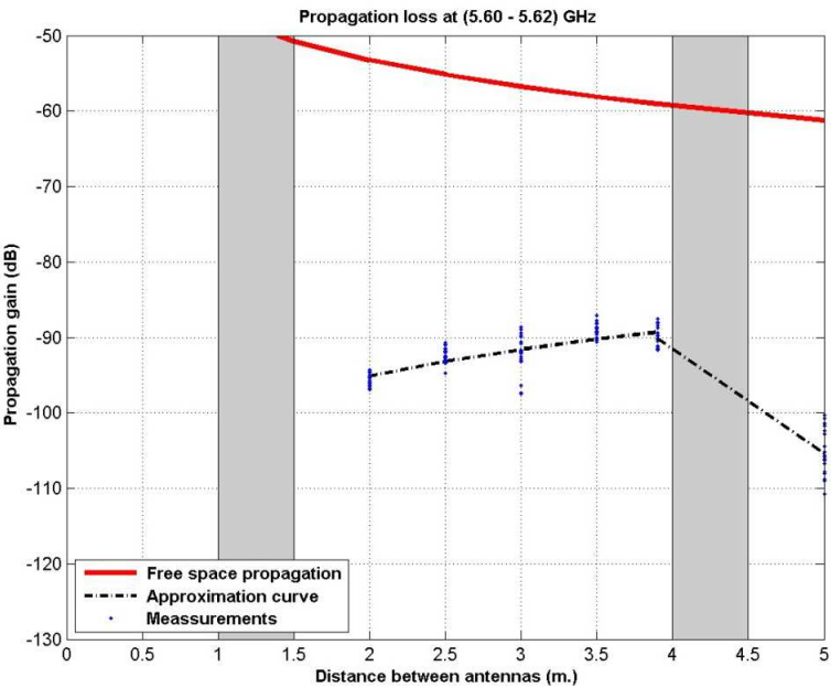
Figure 12. Propagation loss due to the second diffraction scenario with vertical polarization and antenna gain of 19 dB at both transmitting and receiving sides.
