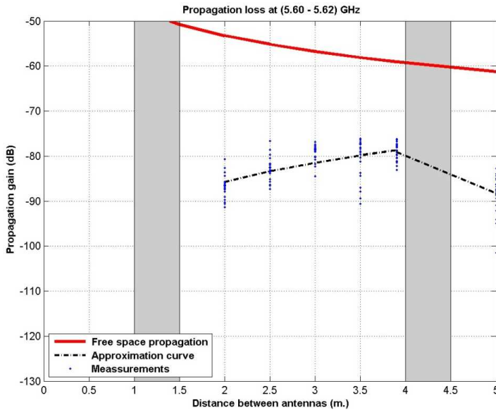
Figure 15. Propagation loss due to the second diffraction scenario with horizontal polarization using a transmitting antenna with a gain of 11 dB and a receiving one with a gain of 8 dB.
