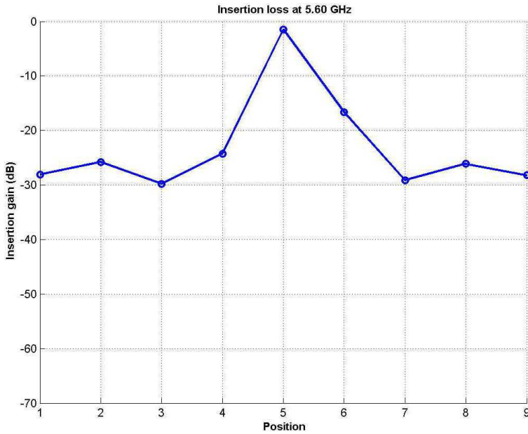
Figure 4. Insertion gain with horizontal polarization using two antennas with a gain of 11 and 8 dB respectively.
