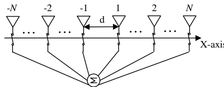
Figure 3. Centro-symmetric thinned linear antenna array.
