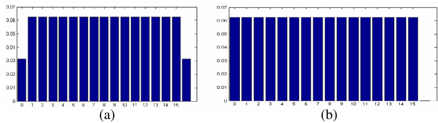
Figure 1. Probability density of each integer value between 0 and 15. (a) Distribution probability of every discrete point using round function. (b) Distribution probability of every discrete point using the rounddown function.
