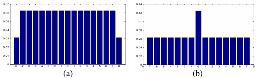
Figure 2. Distribution probability of each integer value between -7 and 7 . (a) Distribution probability of every discrete point using round function. (b) Distribution probability of every discrete point using the rounddown function.
