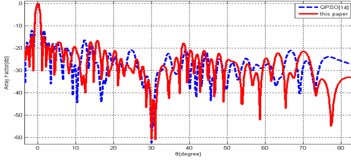
Figure 8. The optimized array pattern with minimum PSLL and null control (solid). 100 elements, null positions are 30^\circ and 31^\circ , PSLL = -14.7 dB, HPBW = 0.8^\circ , directivity = 24.2 dB.
