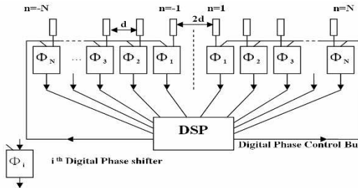
Figure 7. Centro-symmetric antenna array using digital phase shifters.
