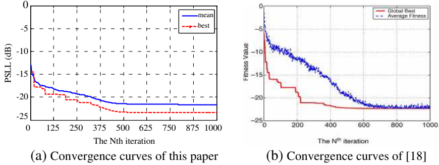
Figure 12. Convergence curves comparison.
