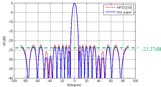
Figure 11. Best result, 20 element, PSLL = -23.27 dB.
