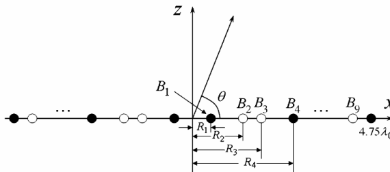
Figure 10. A symmetric aperiodic thinned array with a dimension of 9.5\lambda and a largest possible element number of 20. The locations and on/off status of isotropic antenna elements are represented by a real vector consisting of 18 real numbers in [0, 1] .
