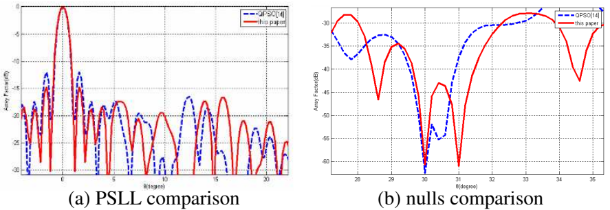
Figure 9. The PSLL comparison of two results.
