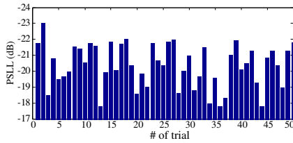
Figure 5. Distribution of PSLLs, 77% filled.
