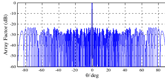
Figure 4. The pattern of result 1 in Table 2. (PSLL = -23.03 dB, fill factor = 77%, HPBW = 0.58^\circ , Directivity = 28.74 dB).
