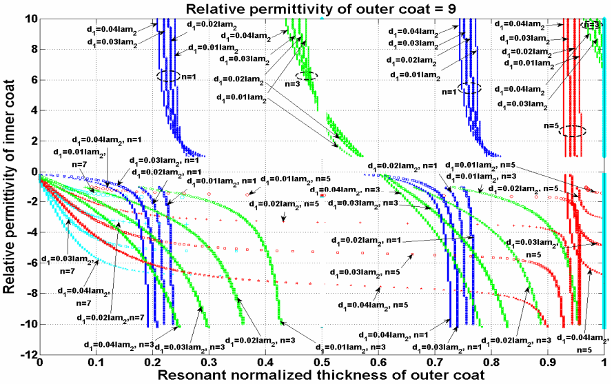
Figure 5. Contour paths of resonances extracted from Figs. 3(b) and 3(e), and several other d_1 cases ( 0.02\lambda_2 , 0.03\lambda_2 , and 0.04\lambda_2 ), for \varepsilon_{r2} = 9 .
