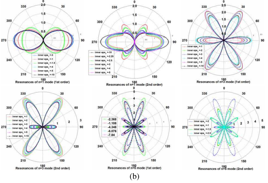
Figure 6. Directive gain patterns (variation with \theta ) generated by (18) for selected points along resonant paths of Fig. 5 (upper cluster) and an additional case of \varepsilon_{r2} = +16 (lower set), for d_1 = 0.01\lambda_2 and \varepsilon_1 < 0 . Each cluster of plots corresponds to a certain \varepsilon_2 , and each subplot within pertains to a certain n th mode. Relative permeability \mu_{r1} = \mu_{r2} = 1 throughout. (a) \varepsilon_{r2} = +9 , d_1 = 0.01\lambda_2 , \varepsilon_1 < 0 (of Fig. 5). (b) \varepsilon_{r2} = +16 , d_1 = 0.01\lambda_2 , \varepsilon_1 < 0 .
