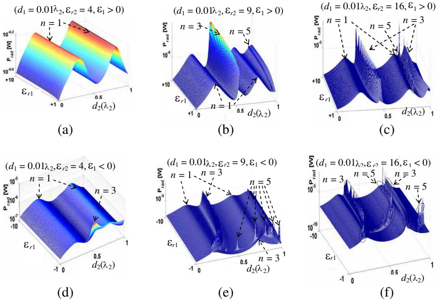
Figure 3. Total radiated power as a function of the permittivity \varepsilon_1 of the inner layer and thickness d_2 of the outer layer, for positive and negative \varepsilon_1 , and various positive relative permittivities \varepsilon_{r2} of the outer layer (4, 9 and 16), as indicated. The outer coat thickness d_2 normalized to its dielectric wavelength \lambda_2 = 1/[f\sqrt{(\mu_2\varepsilon_2)}] ranges from 0 to 1. Inner coat thickness d_1 = 0.01\lambda_2 . Cases (a) to (c) are for \varepsilon_1 > 0 , cases (d) to (f) are for \varepsilon_1 < 0 . Relative permeability \mu_{r1} = \mu_{r2} = 1 throughout.
