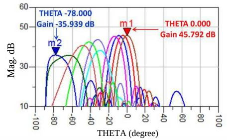
Figure 13. The 8 \times 8 planar array beam steering.
