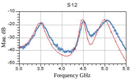
Figure 6. The 1 \times 2 array coupling coefficients.
