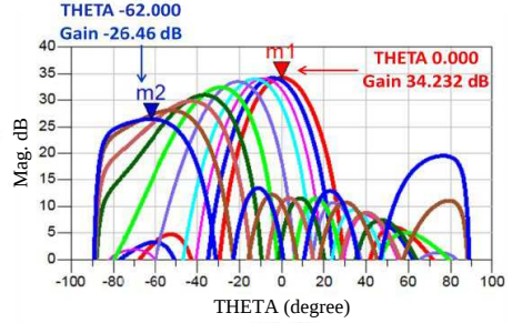
Figure 11. The 4 \times 4 planar array beam steering.
