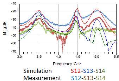
Figure 9. The 1 \times 4 array coupling coefficients S_{12} , S_{13} , S_{14} .
