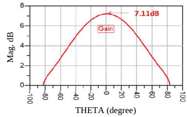
Figure 3. Single element gain.
