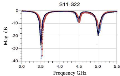
Figure 5. The 1 \times 2 array reflection coefficients.
