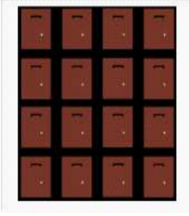
Figure 10. The compact dual-band planar 4 \times 4 U-slotted rectangular patch array antenna.
