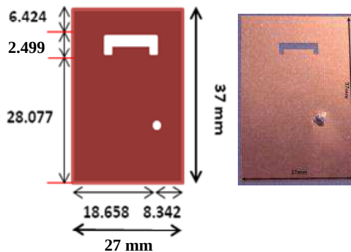
Figure 1. Geometry of a U-slotted antenna element.
