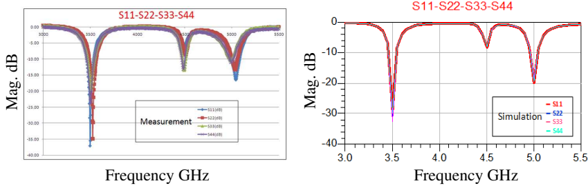
Figure 8. The 1 \times 4 array reflection coefficients S_{11} , S_{22} , S_{33} , S_{44} for measurement and simulation.
