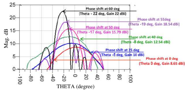
Figure 14. Gains with different steer angles at different phase shift angles.
