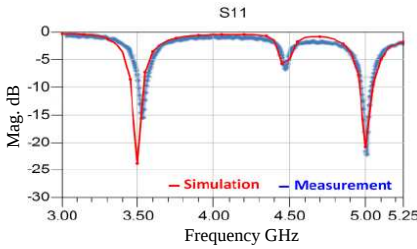
Figure 2. Single element reflection coefficient S_{11} .
