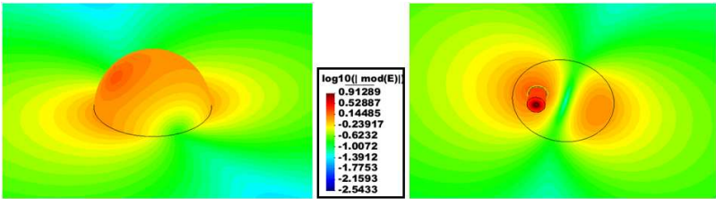
Figure 6. Electric field at f = 3.65 GHz calculated with ERMES for the hemispherical dielectric resonator antenna.
