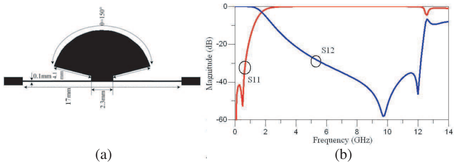
Figure 2. (a) The proposed suppressing cell. (b) The frequency response of the suppressing cell.
