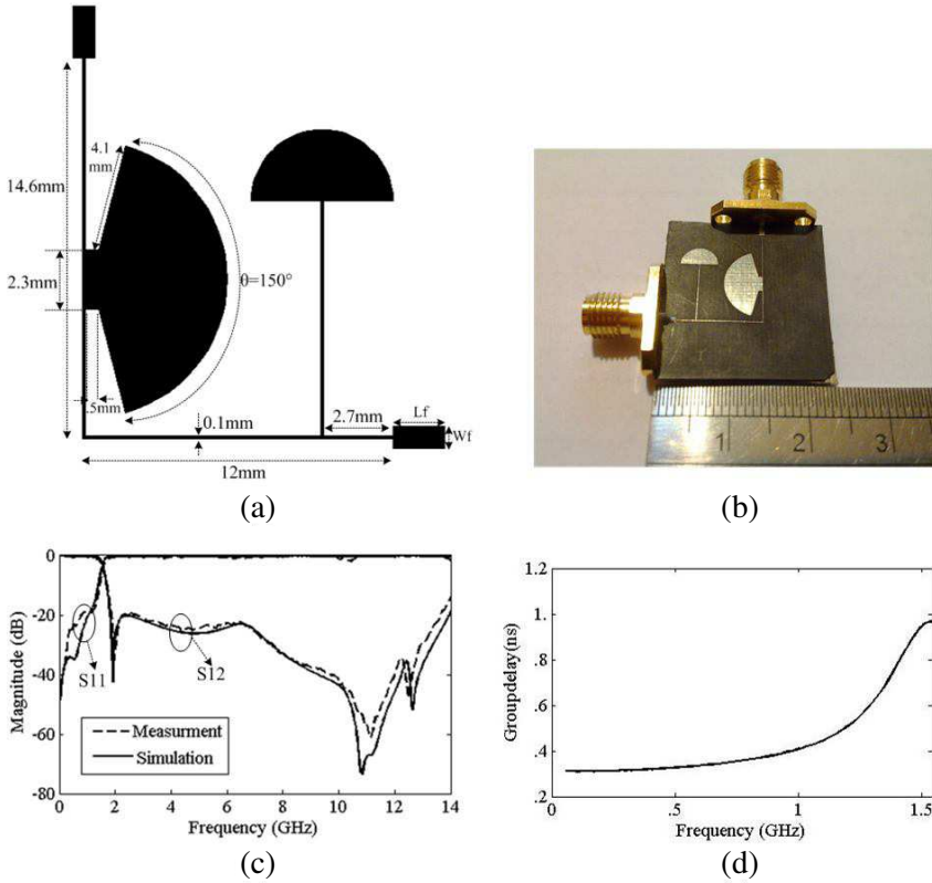
Figure 3. (a) Schematic of proposed lowpass filter. (b) Photograph of fabricated lowpass filter. (c) Simulation and measurement results of the designed lowpass filter. (d) Group delay of the proposed lowpass filter.
