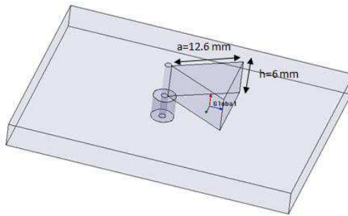
Figure 1. Equilateral TDRA.
