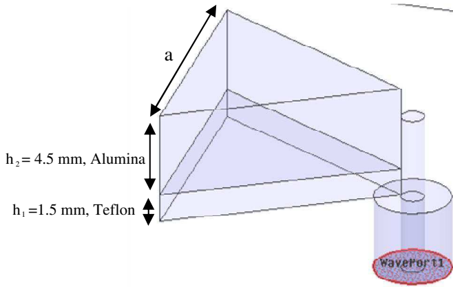
Figure 3. Single element dual segmented TDRA.
