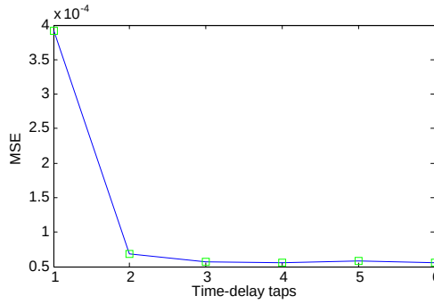
Figure 7. MSE variation versus the number of time-delay taps of OHPBNN PA behavioral model.
