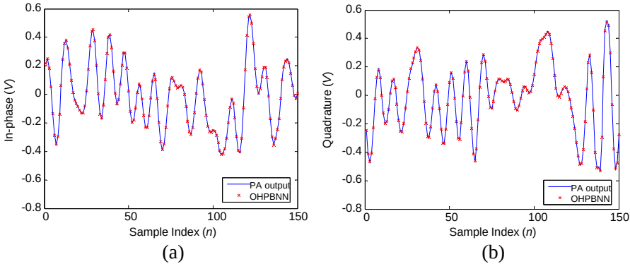
Figure 12. Time-domain validation for OHPBNN model. (a) In-phase component. (b) Quadrature component.
