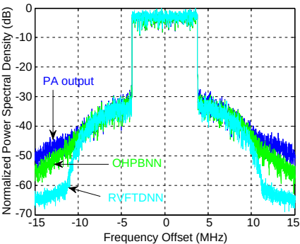
Figure 8. PSD comparison for the PA output, OHPBNN model and RVFTDNN model prediction.
