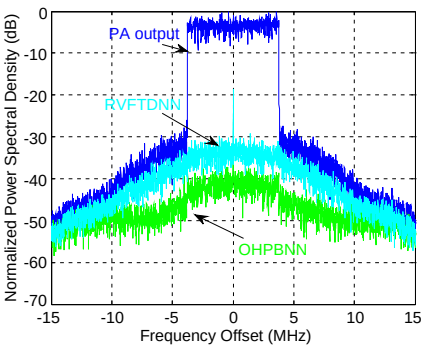
Figure 9. PSD of the error signals both for the OHPBNN and RVFTDNN.
