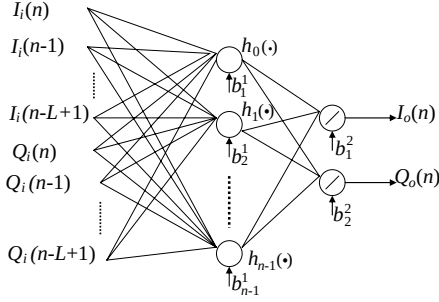
Figure 5. OHPBNN PA behavioral model.
