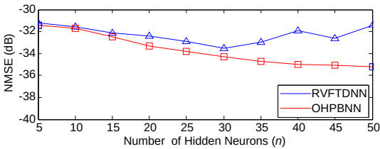
Figure 10. NMSE variation versus the number of hidden neurons both for OHPBNN and RVFTDNN model.
