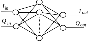
Figure 3. RVFFNN neural network.
