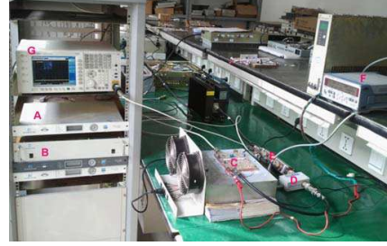
Figure 6. Test platform.
