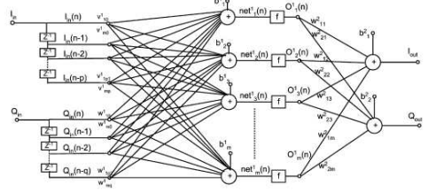
Figure 4. RVFTDNN neural network.
