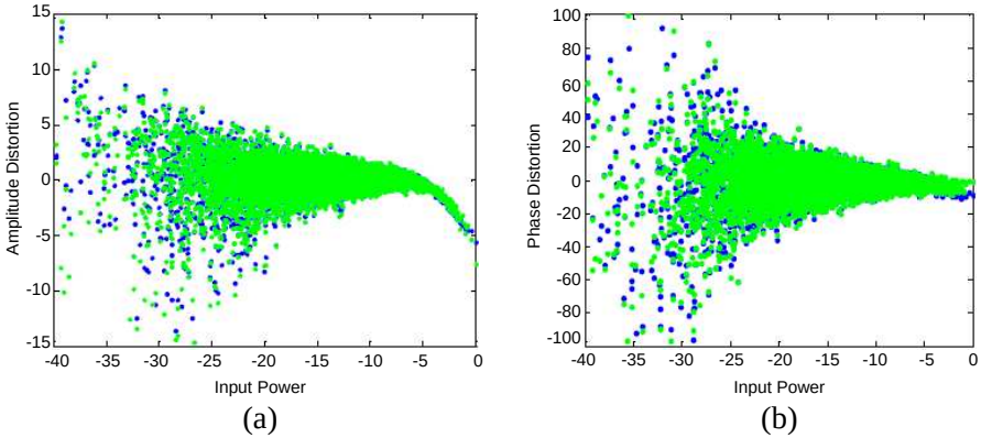
Figure 11. Dynamic nonlinear AM/AM and AM/PM characteristic comparison between the PA output and OHPBNN prediction. (a) AM/AM. (b) AM/PM.
