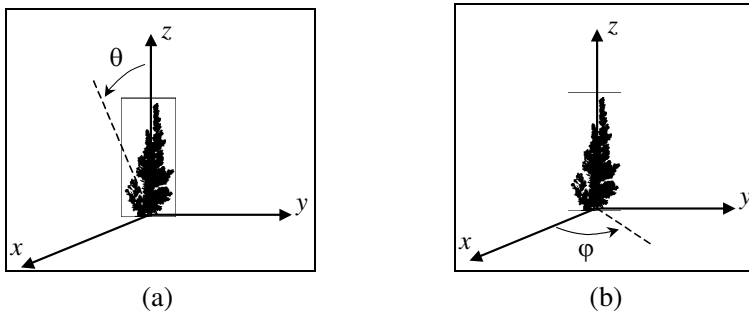
Figure 7. Measurement configuration in (a) xz -plane, \varphi = 0 and (b) xy -plane, \theta = 90 .
