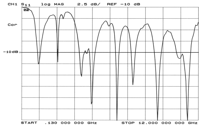
Figure 2. Return loss of the branched tree-like monopole.
