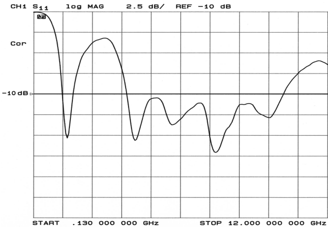
Figure 3. Return loss of the planar monopole with fractal contour.
