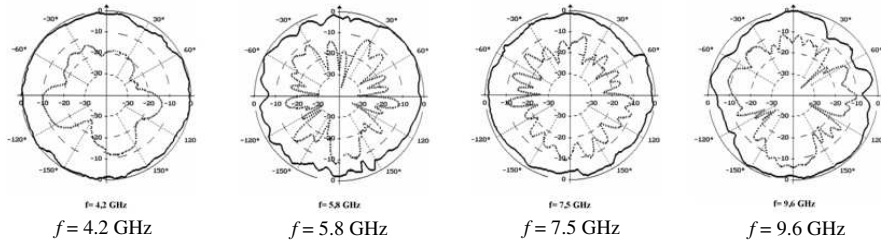
Figure 6. Radiation patterns of the planar monopole with fractal contour in the xy -plane at resonant frequencies 4.2, 5.8, 7.5, and 9.6 GHz. — E_\theta , --- E_\phi .
