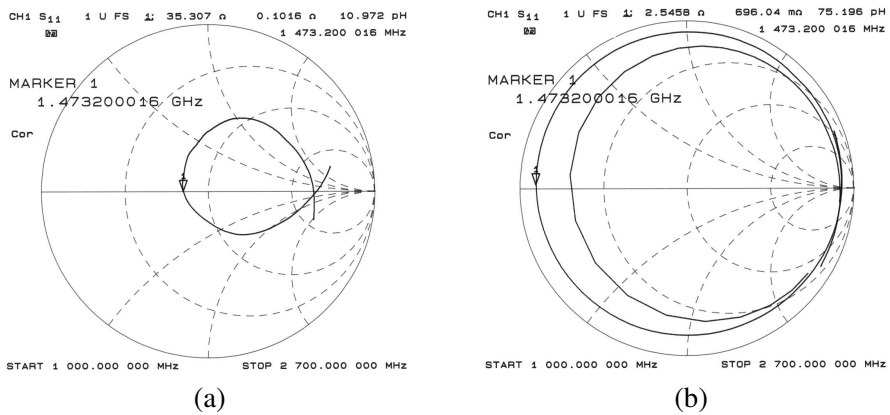
Figure 4. Input impedance Smith chart of the planar structure with fractal contour: (a) in free space and (b) enclosed by the cap.
