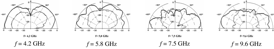
Figure 5. Radiation patterns of the planar monopole with fractal contour in the xz -plane at resonant frequencies 4.2, 5.8, 7.5, and 9.6 GHz. — E_\theta , - - - E_\phi .
