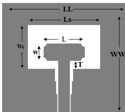
Figure 1. Geometry of the prototype antenna.
