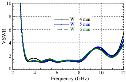
Figure 5. Effects of the stub width W on the VSWR.
