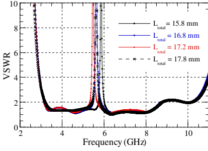
Figure 8. VSWR for various lengths of L_{total} of C-slot.
