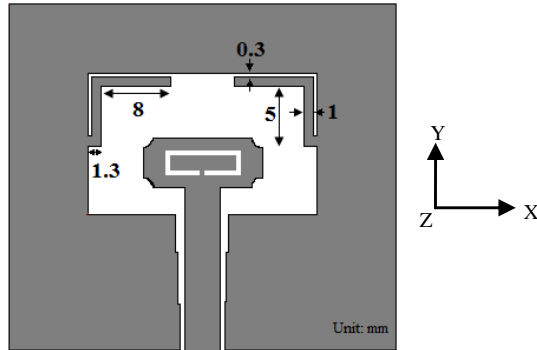
Figure 3. Geometry of proposed antenna with C-slot and L-shape stubs.
