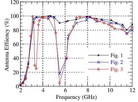
Figure 20. Frequency vs. antenna efficiency plot.
