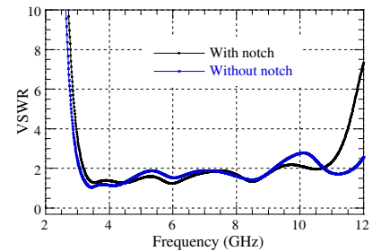
Figure 7. Simulated VSWR with and without notch in ground plane.
