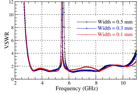
Figure 9. VSWR for various width of C-slot.
