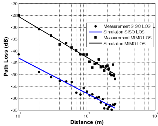
Figure 4. Path loss versus distance in LOS scenario.
