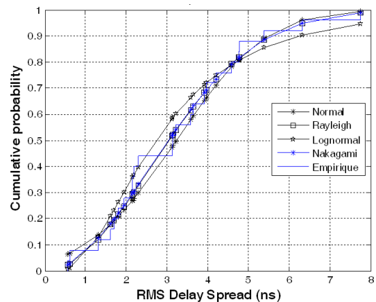
Figure 9. Cumulative distribution function of the RMS and different distributions.
