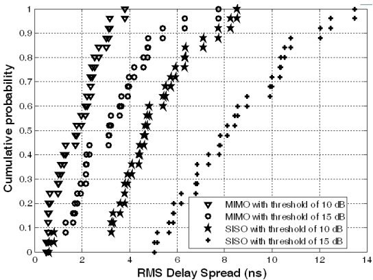
Figure 7. Cumulative distribution function for two thresholds for MIMO and SISO in LOS.
