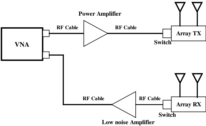
Figure 2. Measurement setup.
