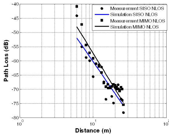
Figure 5. Path loss versus distance (dB) in NLOS scenario.
