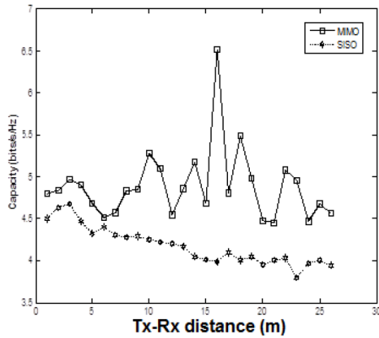
Figure 10. Comparison of the capacity for MIMO and SISO in LOS condition.
