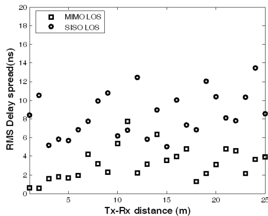
Figure 8. Comparison of the delay spread for MIMO and SISO for a threshold of 15 dB in LOS.
