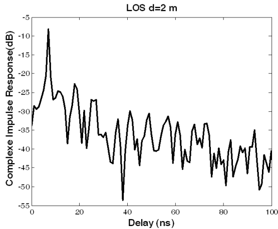
Figure 6. Example of power delay profile for MIMO at 2 m in LOS.
