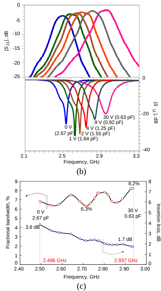
Figure 6. The measured S -parameters of the reconfigurable microstrip LC bandpass filter. (a) The simulated and measured S -parameters under 0 V and 30 V bias. (b) The measured S -parameters under various bias voltages. (c) The fractional bandwidth and insertion loss versus the central frequency of the reconfigurable filter.
