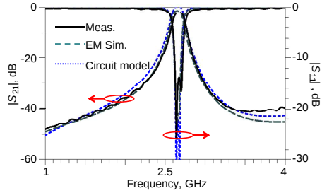
Figure 3. Simulated, measured and circuit model calculated S -parameters of the microstrip LC bandpass filter.
