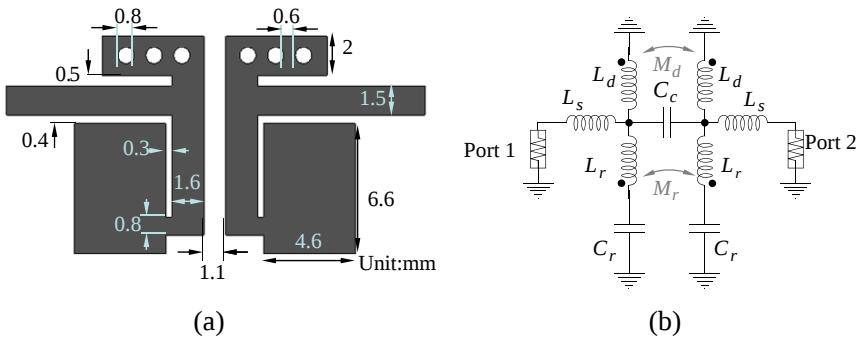
Figure 1. (a) Layout and (b) lumped equivalent circuit model of the microstrip LC bandpass filter.
