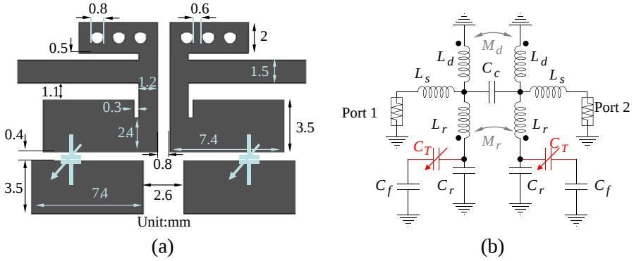
Figure 4. (a) Layout and (b) lumped equivalent circuit model of the reconfigurable microstrip LC bandpass filter.
