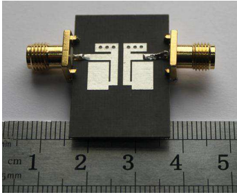
Figure 2. Fabricated bandpass filter based on mix coupled microstrip LC resonator.
