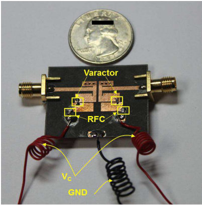
Figure 5. Fabricated reconfigurable microstrip LC bandpass filter based on semiconductor varactor diode.
