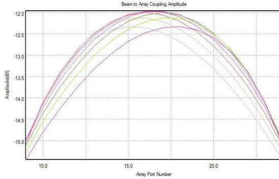
Figure 4. Satellite Rotman lens computed beam to array coupling amplitude.
