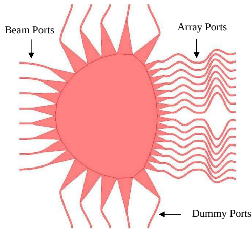
Figure 2. Layout of the proposed satellite 8 \times 16 Rotman lens for the operating frequency of 14.5 GHz. The MBFN lens includes input beam ports; array-receiving ports; and dummy ports (each is terminated by a 50\text{-}\Omega load).
