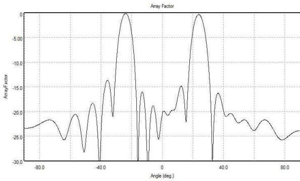
Figure 6. Satellite Rotman lens computed AF radiation pattern with beam port 1 and beam port 8 excited for aperture distribution beam scanning.
