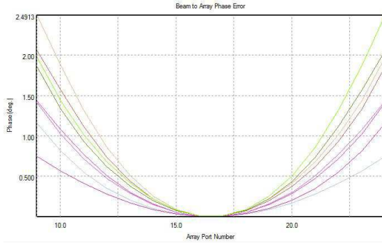
Figure 3. Satellite Rotman lens computed beam to array phase error.
