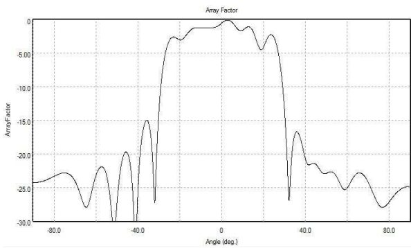
Figure 5. Satellite Rotman lens computed array factor radiation pattern.
