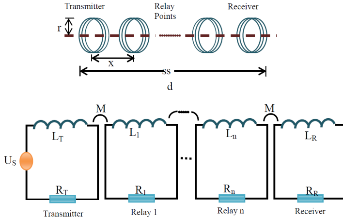
Figure 4. Magnetic waveguide and its circuit model.
