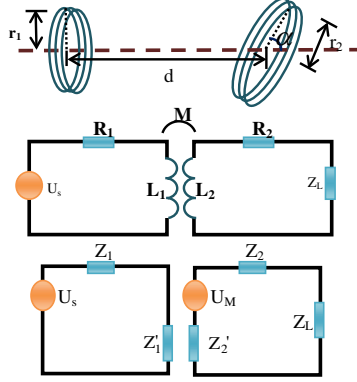
Figure 1. MI communication system.
