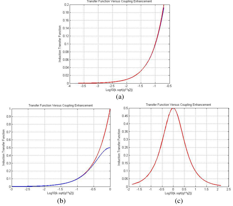
Figure 2. Compared transfer functions with/without approximation ( N = 2 ). (a) Compared transfer function at low Q (red curve is with approximation; blue curve has no approximation). (b) Compared transfer function at high Q , with approximation (read curve); without approximation (blue curve). (c) Variation of transfer function with Q .
