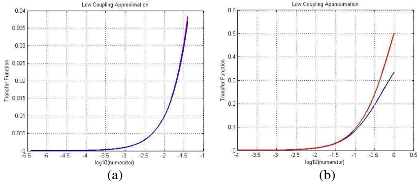
Figure 3. Power transfer functions with approximation ( N = 3 ). (a) Power transfer function when Q = 2 ; Red = approximation; Blue = no approximation. (b) Power transfer function when Q = 10 ; Red = approximation; Blue = no approximation.
