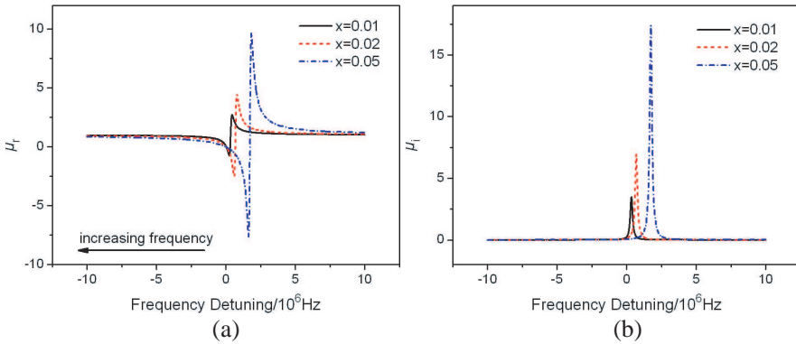
Figure 2. The relation between magnetic permeability of (Yb_xY_{1-x})_3Al_5O_{12} crystal and frequency detuning. (a) \mu_r , real part of magnetic permeability. (b) \mu_i , imaginary part of magnetic permeability. The concentrations of Yb^{3+} ion are x = 0.01, 0.02 and 0.05 respectively.
