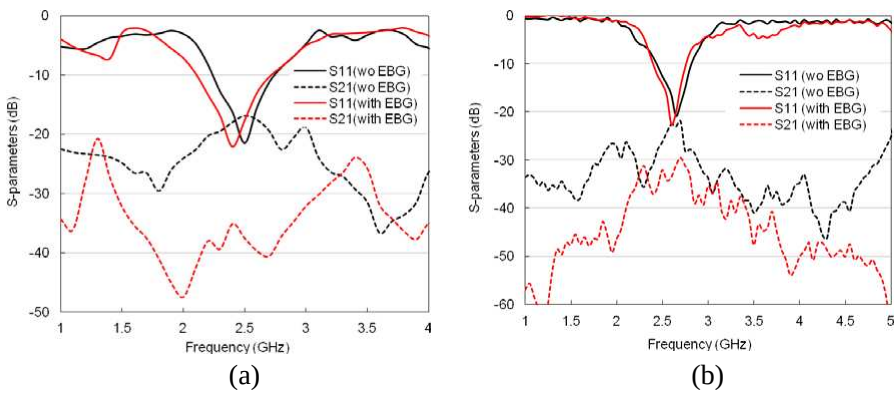
Figure 7. Scattering parameters of the patch antenna array, (a) simulated, and (b) measured.
