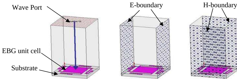
Figure 4. Simulation model for reflection phase analysis.
