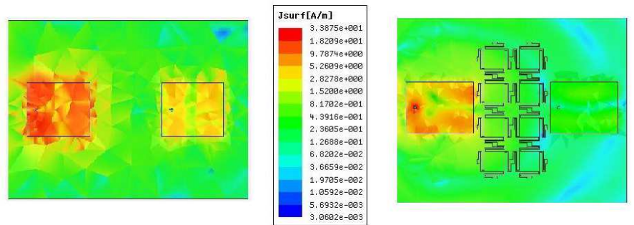
Figure 8. Surface current distribution with and without EBG structure.
