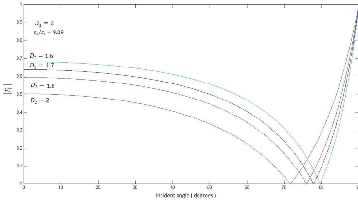
Figure 16. Change in magnitude of reflection coefficient and Brewster's angle for parallel polarization for varying dimension, D_2 .
