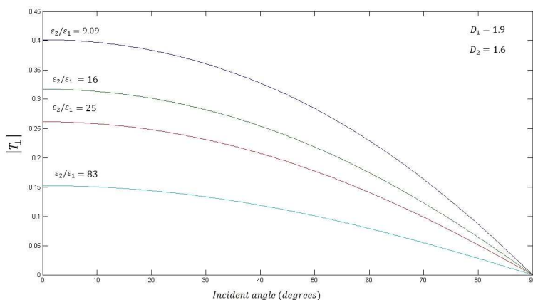
Figure 6. Magnitude of transmission coefficients for perpendicular polarization for non-integer dimension space.
