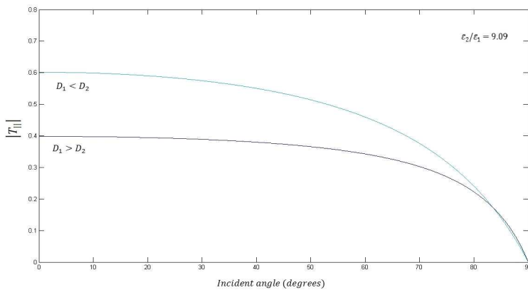
Figure 11. Magnitude of transmission coefficients for parallel polarization for varying dimension D_1 and D_2 .
