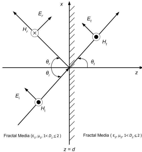
Figure 1. Parallel polarized wave at dielectric fractal-fractal interface.
