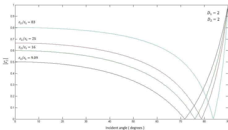
Figure 7. Magnitude of reflection coefficients for parallel polarization for integer dimension space.
