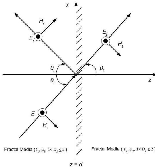
Figure 2. Perpendicular polarized wave at dielectric fractal-fractal interface.
