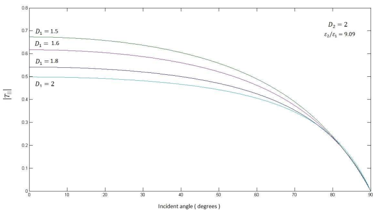
Figure 13. Magnitude of transmission coefficients for parallel polarization for varying dimension D_1 .
