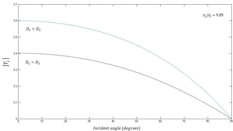
Figure 12. Magnitude of transmission coefficients for perpendicular polarization for varying dimension D_1 and D_2 .
