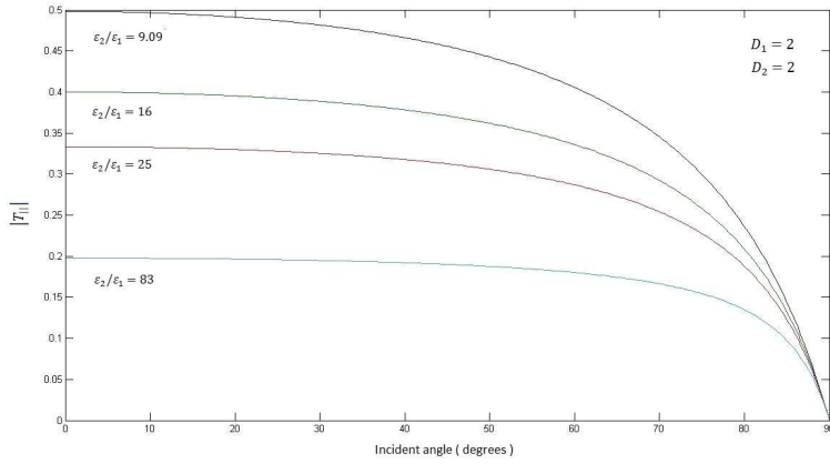
Figure 8. Magnitude of transmission coefficients for parallel polarization for integer dimension space.
