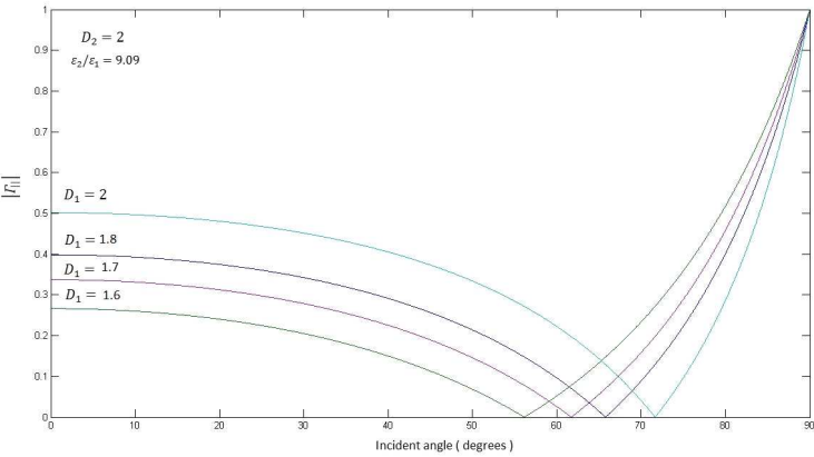
Figure 15. Change in magnitude of reflection coefficient and Brewster's angle for parallel polarization for varying dimension, D_1 .
