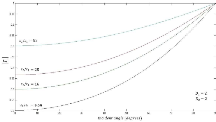
Figure 9. Magnitude of reflection coefficients for perpendicular polarization for integer dimension space.
