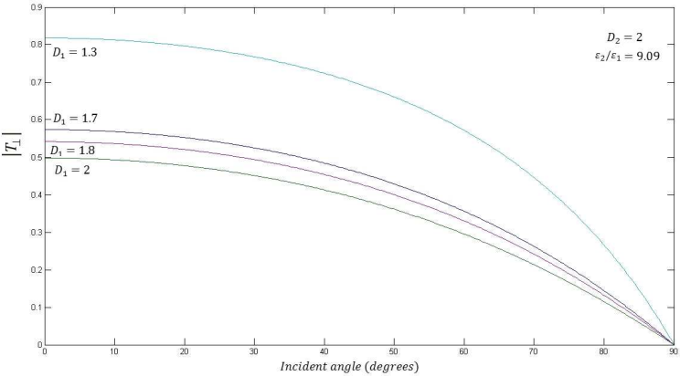
Figure 14. Magnitude of transmission coefficients for perpendicular polarization for varying dimension D_1 .
