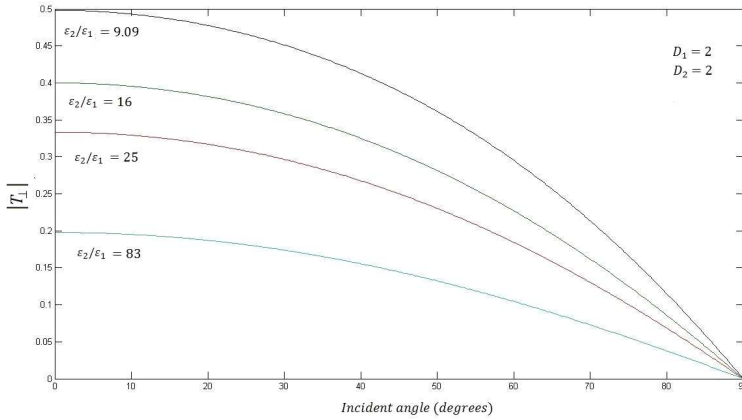
Figure 10. Magnitude of transmission coefficients for perpendicular polarization for integer dimension space.
