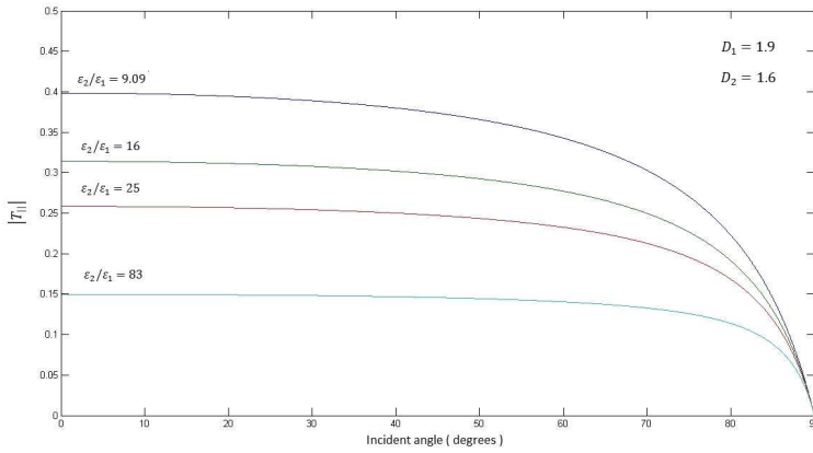
Figure 4. Magnitude of transmission coefficients for parallel polarization for non-integer dimension space.
