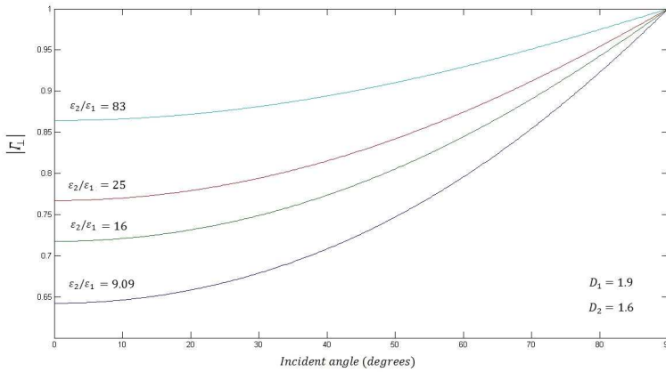
Figure 5. Magnitude of reflection coefficients for perpendicular polarization for non-integer dimension space.
