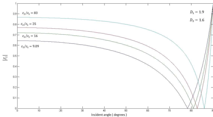
Figure 3. Magnitude of reflection coefficients for parallel polarization for non-integer dimension space.
