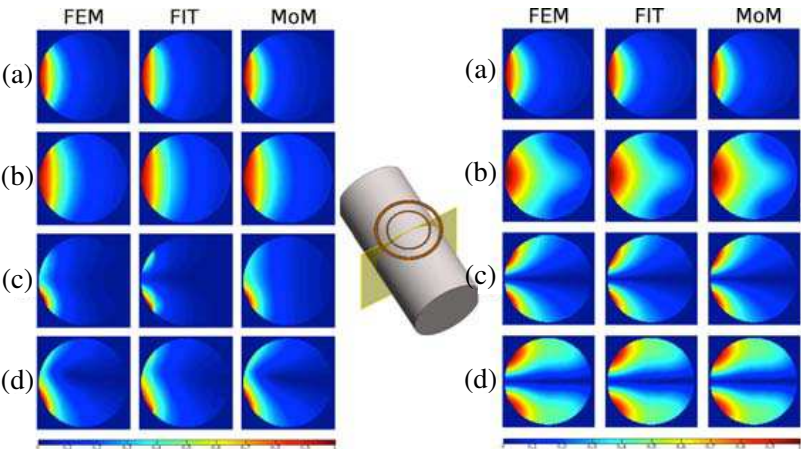
Figure 3. (a), (b) Transverse magnetic field simulated at 120.6 MHz ( ^{31}\text{P} Larmor frequency) and 298.0 MHz ( ^1\text{H} Larmor frequency) respectively on a transverse plane; (c), (d) Electric field simulated at 120.6 MHz and at 298.0 MHz respectively on a transverse plane: the left and right images are referred to the unloaded condition and loaded condition respectively.
