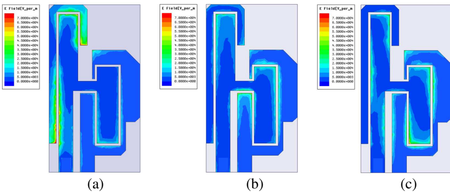
Figure 4. Simulated surface current distribution of the proposed antenna. (a) f = 2.45 GHz, (b) f = 3.5 GHz, (c) f = 5.5 GHz.
