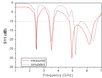
Figure 3. Simulated and measured S_{11} for the proposed antenna.
