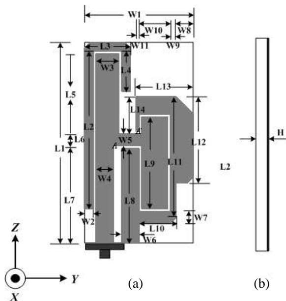
Figure 1. Geometry of the proposed antenna. (a) Top view, (b) side view.
