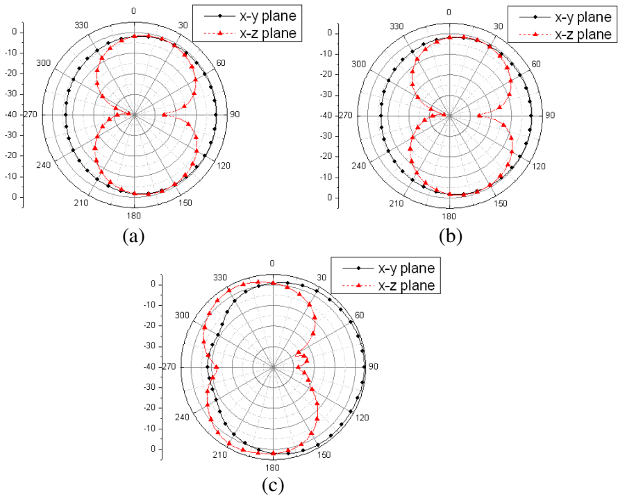
Figure 7. Measured radiation patterns for the proposed antenna. (a) f = 2.45 GHz, (b) f = 3.5 GHz, (c) f = 5.5 GHz.
