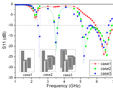
Figure 5. Simulated S_{11} for the proposed antenna in the different cases.
