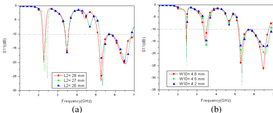
Figure 6. Simulated S_{11} variations for the proposed antenna of different lengths. (a) L2 , (b) W10 .
