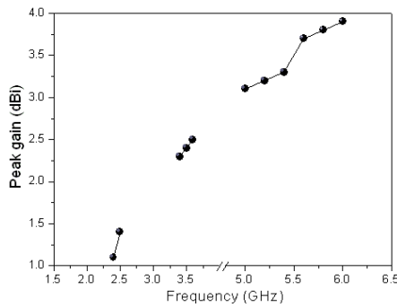
Figure 8. Peak antenna gains for the proposed antenna.
