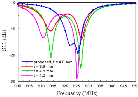
Figure 6. The effect of high-dielectric ceramic substrate thickness on S_{11} response.
