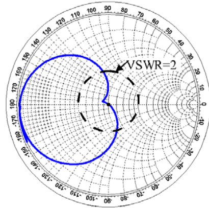
Figure 8. Measured input impedance on Smith Chart of the proposed antenna.
