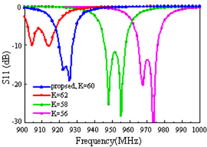
Figure 5. The effect of dielectric constant on S_{11} response.
