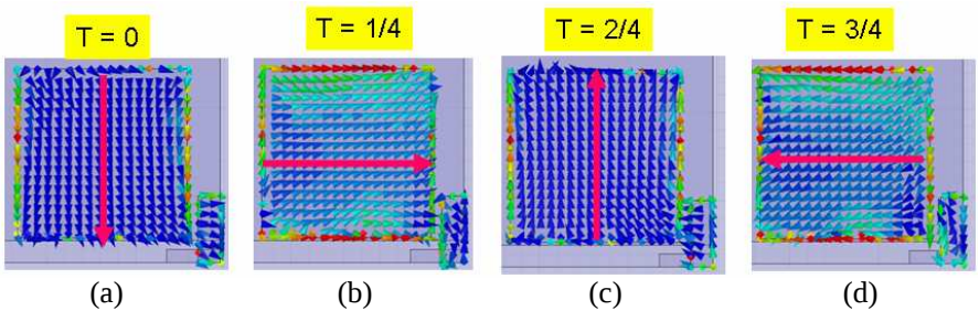
Figure 9. Simulated current distributions of the proposed antenna design. (a) T = 0 , (b) T = 1/4 , (c) T = 2/4 , (d) T = 3/4 .
