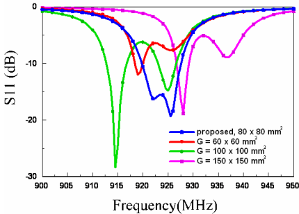
Figure 4. The dimension effect of system ground planes on S_{11} response.
