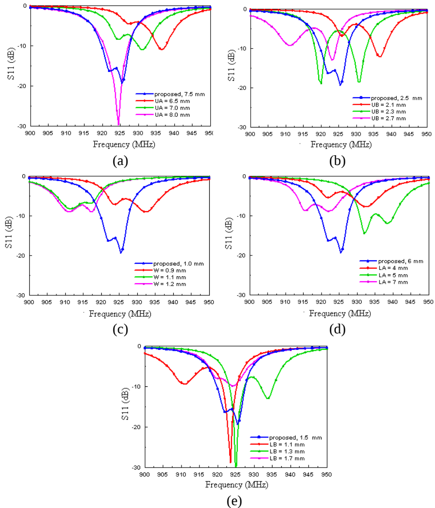
Figure 3. The effects of the multi-bending feeding strip on S_{11} response. (a) UA , (b) UB , (c) W , (d) LA , and (e) LB .
