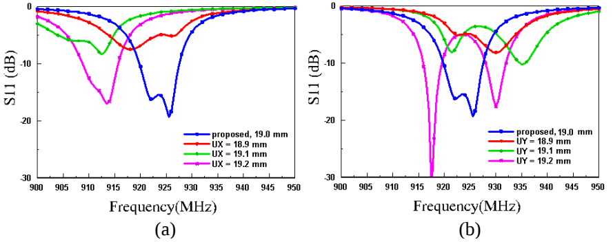
Figure 2. The effects of the top patch size. (a) UX , (b) UY .
