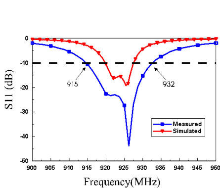
Figure 7. The return loss plot of the patch antenna with novel corner-coupling feed.
