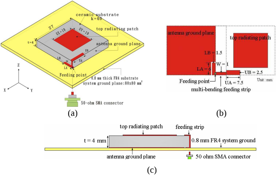
Figure 1. The geometry of proposed antenna. (a) 3-D view, (b) 2-D extending patterns, and (c) side view of the proposed antenna.
