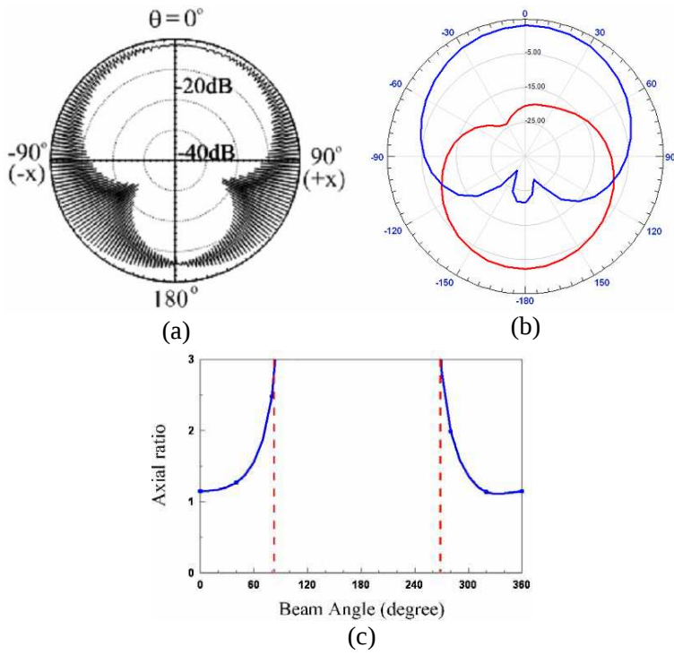
Figure 10. Radiation patterns in x - z plane. (a) Simulated results in RHCP/LHCP components, (b) measured results in circular polarization, and (c) measured 3-dB axial ratio.
