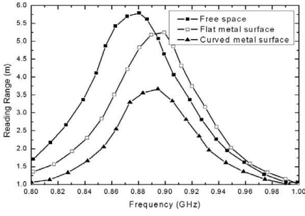
Figure 7. Measured read range of the proposed antenna on flat and curved metallic surfaces (bending radian is about 25 degree) and in free space.
