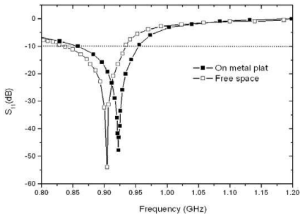
Figure 6. The comparison of input reflection coefficient ( S_{11} ) for the proposed antenna in free space and on a 150 \times 150 \times 8 \text{ mm}^3 metal plate.
