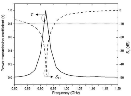
Figure 3. The power transimission coefficient and S_{11} of the proposed antenna on a 150 \times 150 \times 8 mm 3 metal plate.
