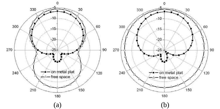
Figure 4. The radiation patterns at 915 MHz in free space and on a 150 \times 150 \times 8 mm 3 metal plate. (a) x - z plane ( \varphi = 0^\circ ). (b) y - z plane ( \varphi = 90^\circ ).
