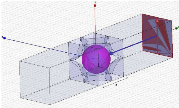
Figure 2. The unit cell model along with the excitation simulated in HFSS, a represents the thickness of the cube.
