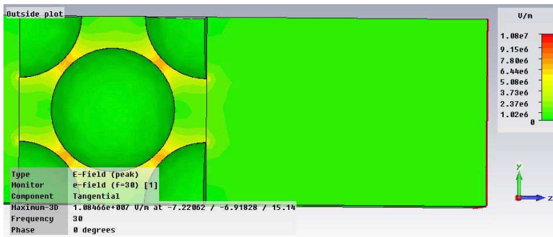
Figure 6. Electric field in the gap region of copper particles at size = 115 \mu\text{m} .
