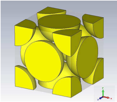
Figure 4. Copper particles arranged in FCC lattice at 70% volume fraction.
