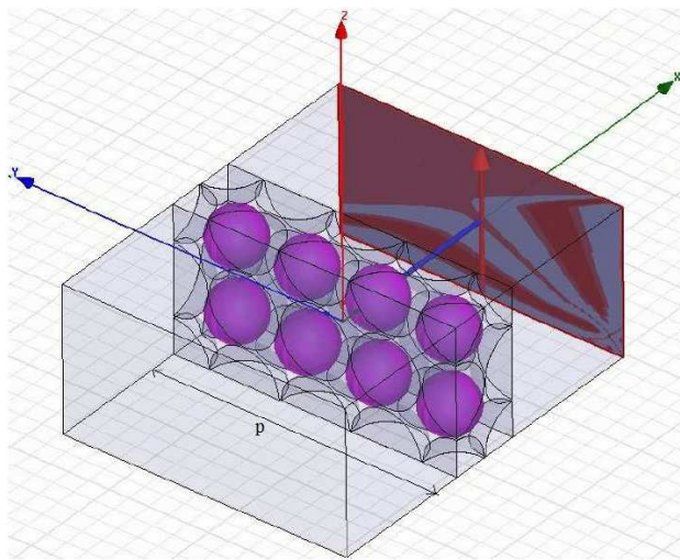
Figure 3. The waveguide model showing a number of unit cells fitted along its cross-section simulated using ANSYS HFSS, p represents the broader dimension of the designated waveguide.
