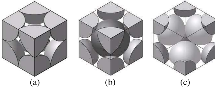
Figure 1. Figures (a) and (b) and (c) show the simple cubic (SC), body centered cubic (BCC) and face centered cubic (FCC) unit cells, respectively.
