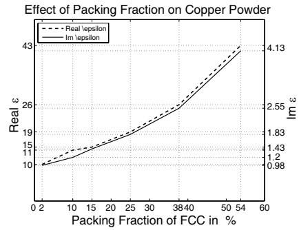
Figure 5. Variation in effective relative permittivity with packing fraction in FCC copper lattice at 30 GHz, at 74% \epsilon_r^* = 7742.441 - 689.291i .
