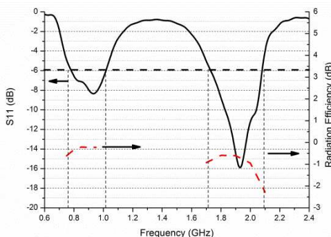
Figure 9. The S -parameter and the radiation efficiency of the modified design.
