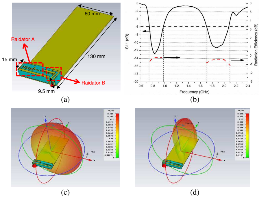
Figure 1. (a) The geometry of the proposed OG PIFA antenna in a mobile handset; (b) S -parameter S_{11} and the radiation efficiency of our antenna; (c) the radiation pattern at 0.8 GHz; and (d) the radiation pattern at 1.8 GHz.
