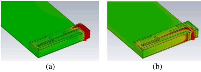
Figure 7. Current distributions of our antenna in free space at (a) 1.8 GHz, (b) 0.8 GHz.
