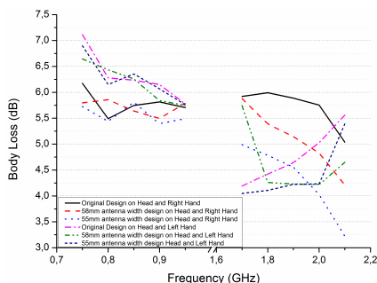
Figure 10. The body loss in the talking mode.
