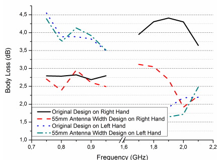
Figure 11. The body loss in the data mode.
