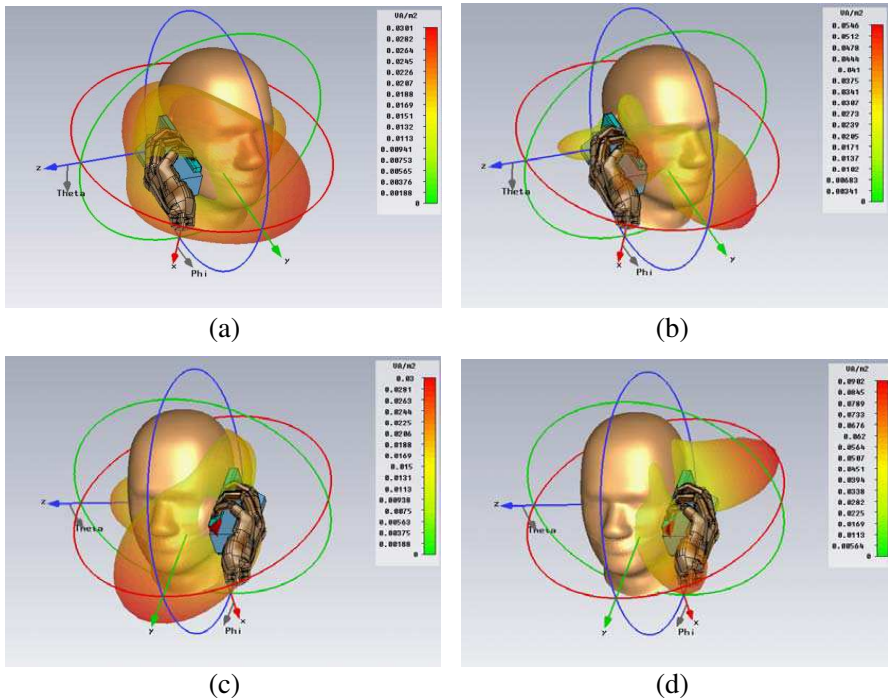
Figure 5. (a) Radiation patterns in the talking position for position 3 at (a) 0.8 GHz, (b) 1.8 GHz with the right hand and at (c) 0.8 GHz, (d) 1.8 GHz with the left hand.
