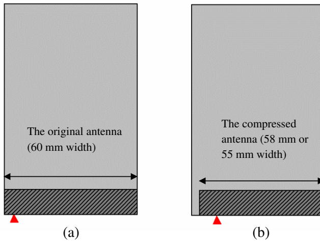
Figure 8. (a) The original design and (b) the modified design.
