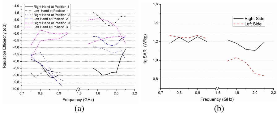
Figure 4. (a) The radiation efficiencies of our antenna in the talking mode, (b) SAR value (according to the 1 g standard) of position 3 on the left or right side of the head phantom.
