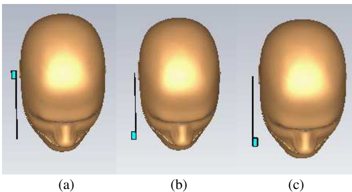
Figure 3. Three different positions of OG PIFA on the right side of the head phantom: (a) position 1, (b) position 2, and (c) position 3.
